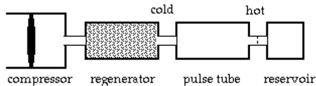
Fig: 1.2 Orifice Pulse Tube
