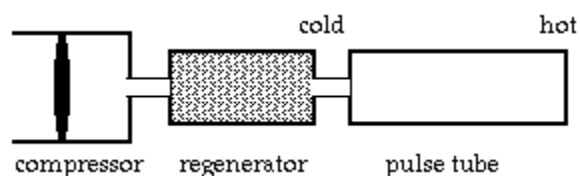
Fig : 1.1 Basic Pulse Tube Refrigerator
