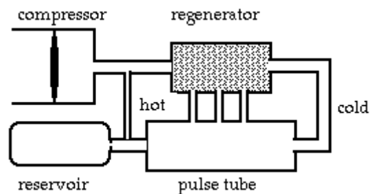
Fig: 1.3 Multiple By-pass Pulse Tube
