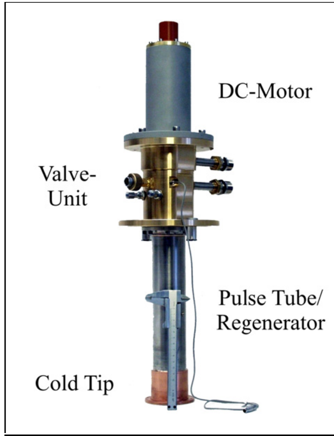
Fig: 4.2 Double Inlet Pulse Tube Refrigerator
