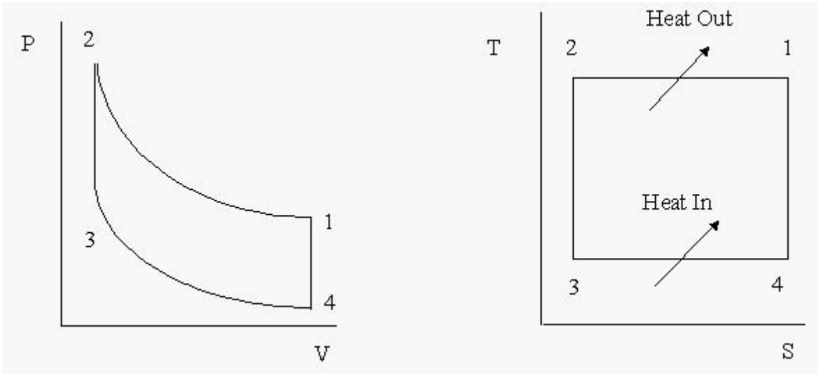
Fig : 2.1 The Stirling Cycle.
