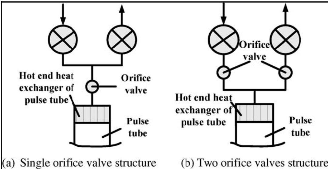
Fig: 4.1 Orifice valve structures
