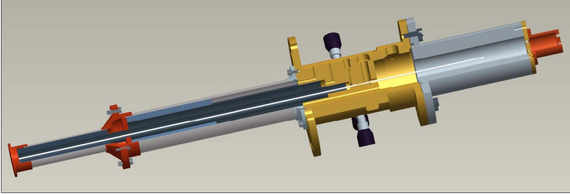
Fig : 3.1 Model of a Grifford-McMahon Refrigerator
