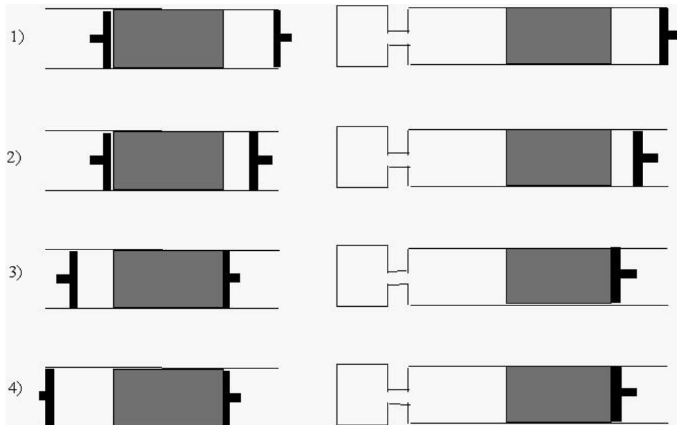
Fig: 2.1 Analogy between pulse tube and Stirling cycle
