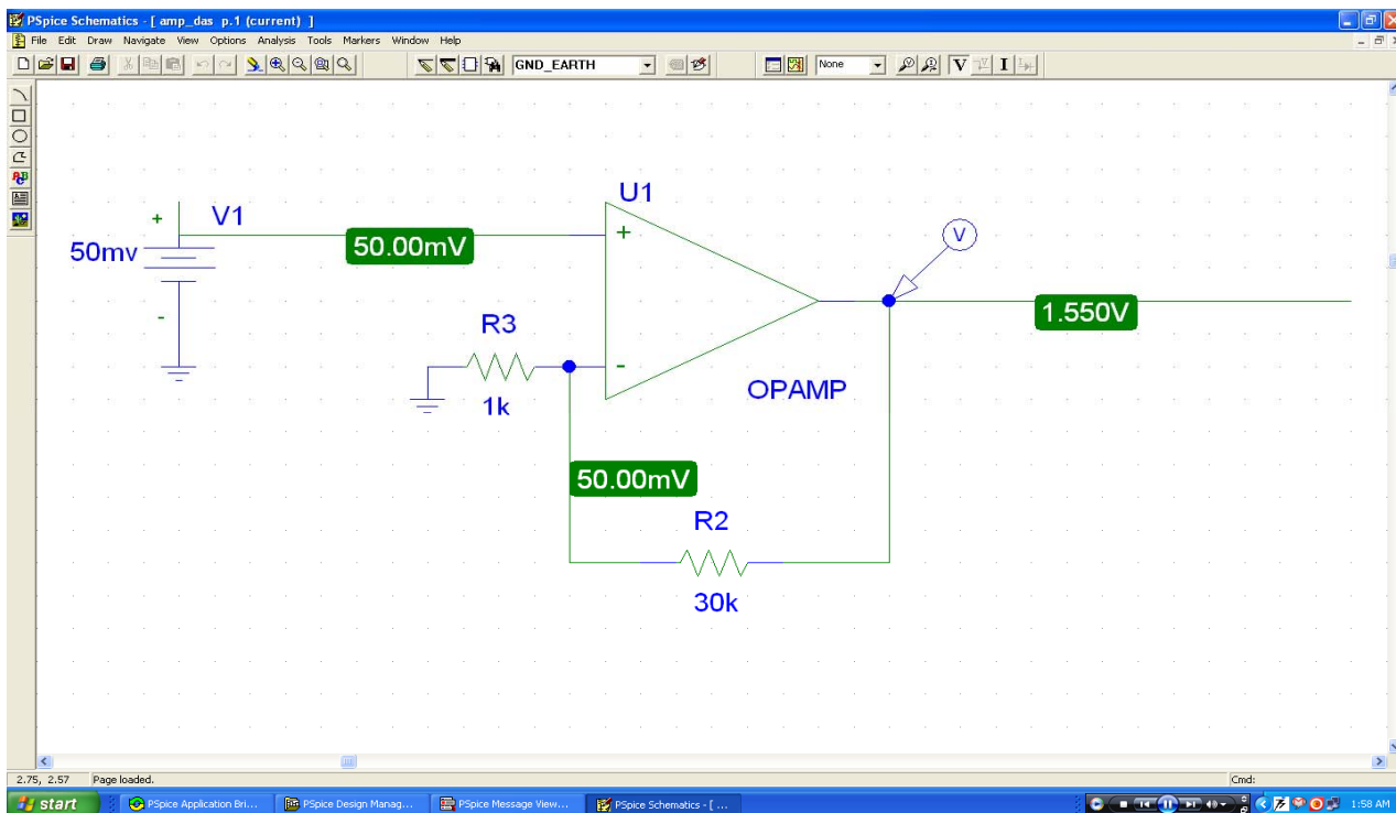
Fig 3.1 :Circuit diagram of amplifying circuit
