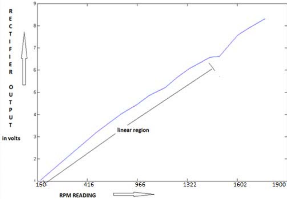
Fig 3.5 rectifiers output vs RPM reading
