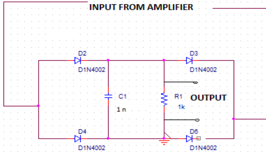
Fig 3.3 CIRCUIT DIAGRAM FOR RECTIFIER
