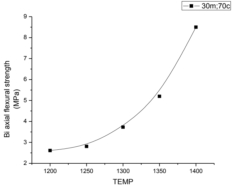
Figure 7b: 30:70 (mullite: cordierite wt %)
