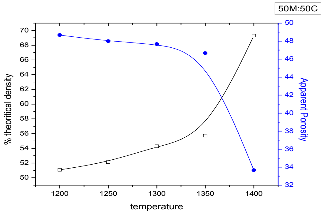
Fig 6c: 50:50(%cordierite: % mullite)
