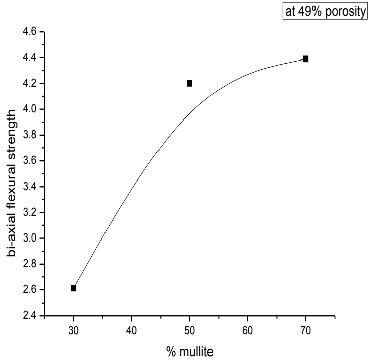
Figure 7 d: % mullite in the composition ~ biaxial flexural strength
