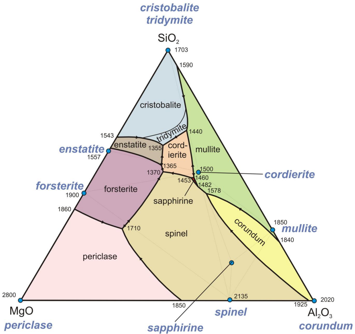
Fig 2: ternary phase diagram for alumina, silica, and magnesia system.
