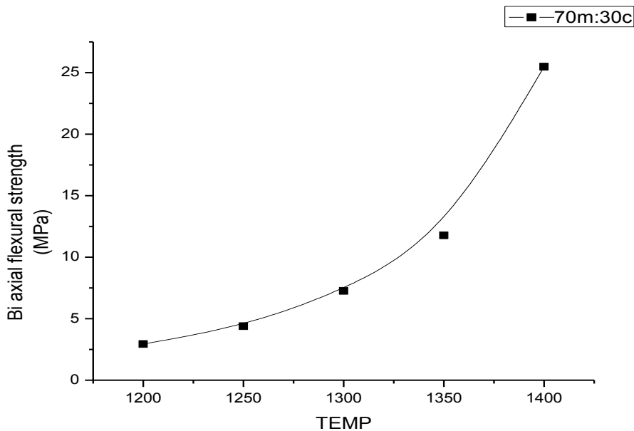
Figure 7a: 70:30 (mullite: cordierite wt %)
