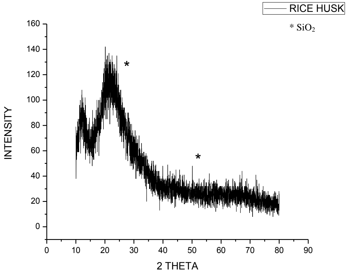
Fig3: XRD pattern of charred rice husk
