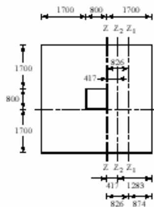
(a) Flexure and one way shear
