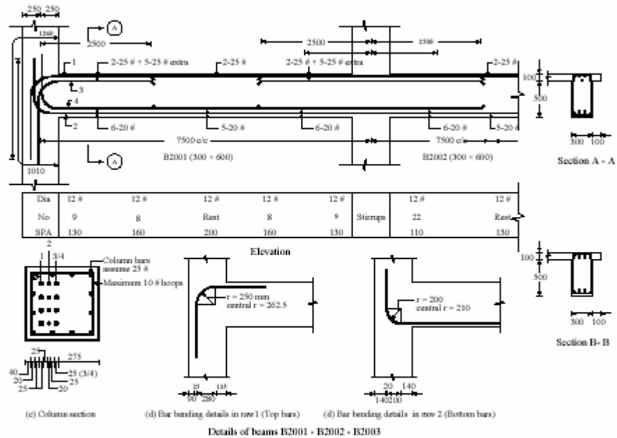
Figure 6 Details of Beams B2001, B2002 and B2003
