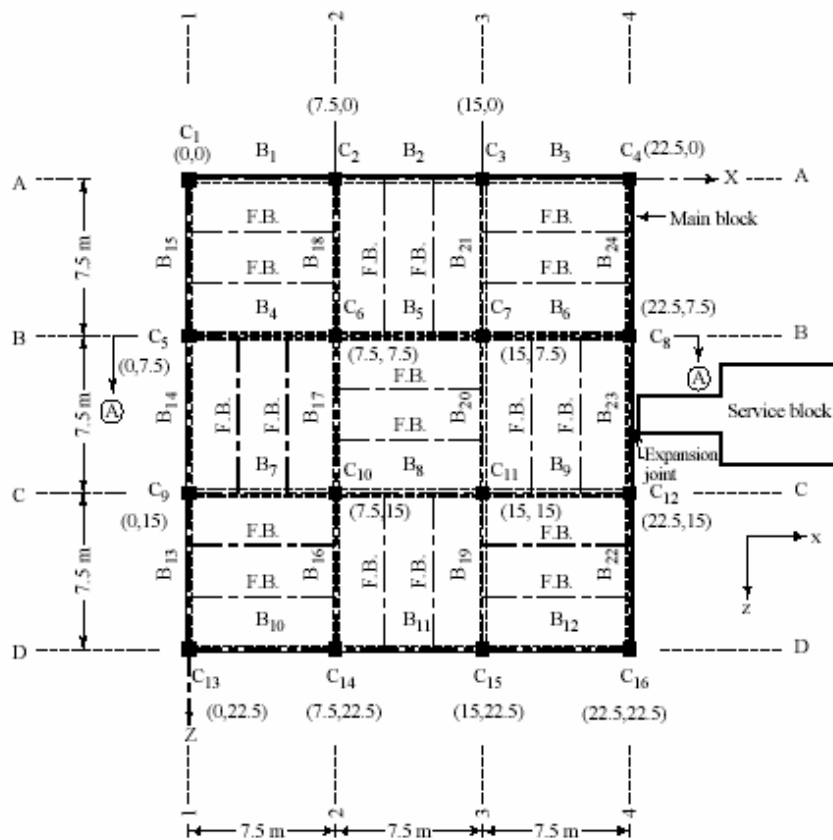
(a) Typical floor plan
