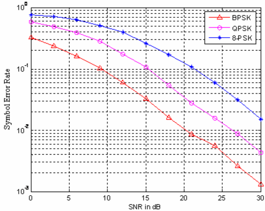
Fig. 5.5: SER (MMSE channel Estimation) for M-PSK modulation for different SNRs
