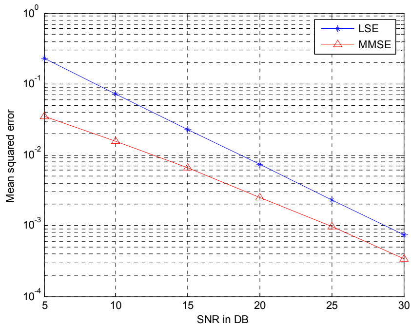
Fig. 5.3: Mean-Square Error for LSE and MMSE estimators at different SNRs.
