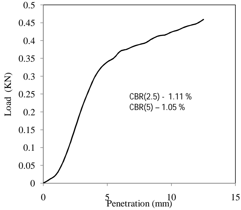
Figure 4.31 Load vs penetration graph for test -5, type -1 soil for soaked (day-4) condition
