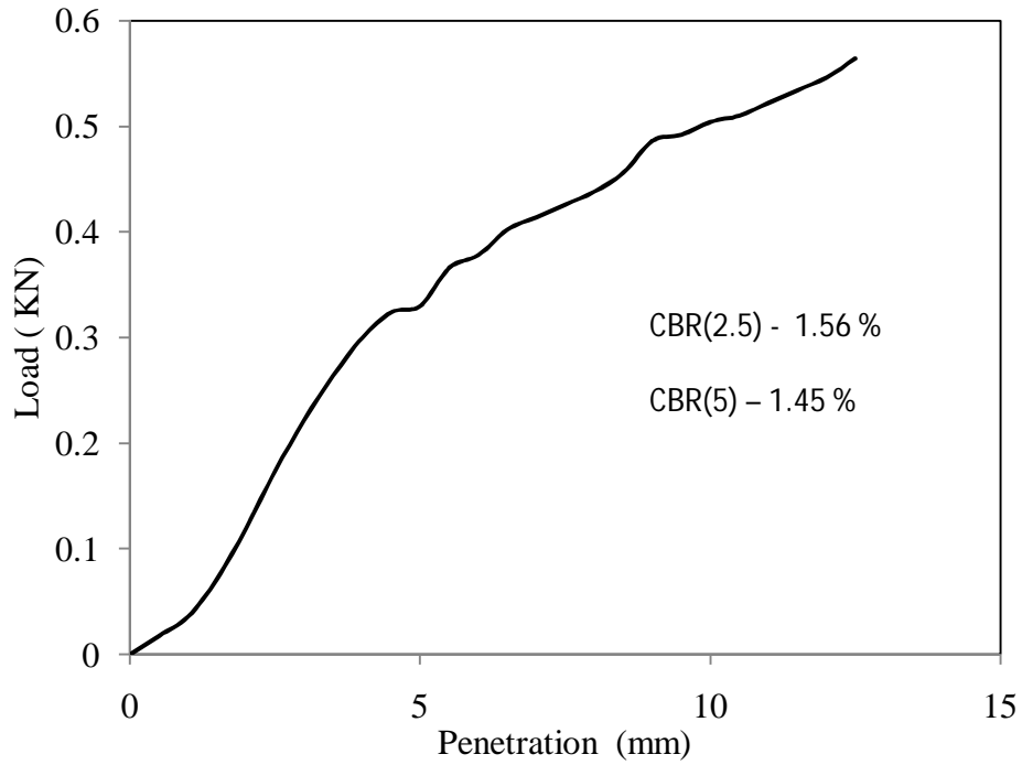
Figure 4.44 Load vs penetration graph for test -2, type -2 soil for soaked (day-4) condition
