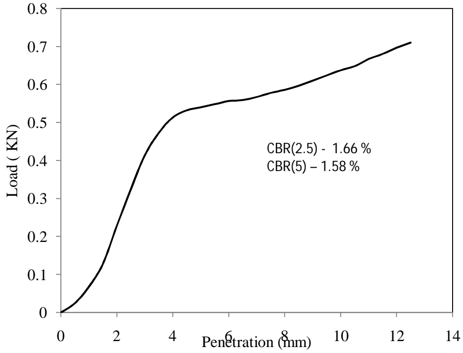
Figure 4.29 Load vs penetration graph for test -5, type -1 soil for soaked (day-2) condition
