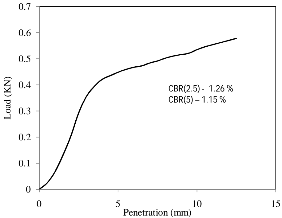
Figure 4.20 Load vs penetration graph for test -3, type -1 soil for soaked (day-5) condition
