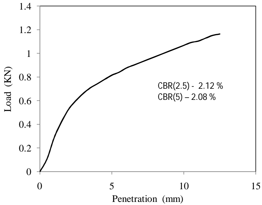
Figure 4.47 Load vs penetration graph for test -3, type -2 soil for soaked (day-1) condition
