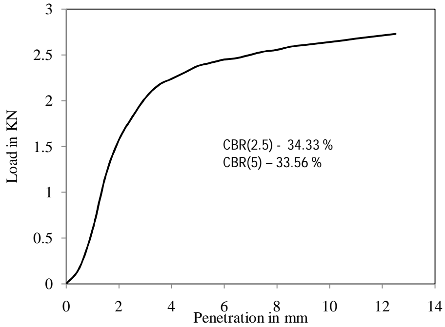
Figure 4.58 Load vs penetration graph for test -5, type -2 soil for unsoaked condition
