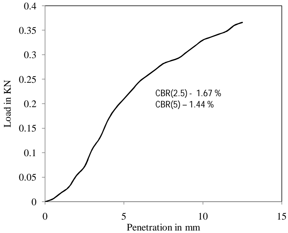
Figure 4.56 Load vs penetration graph for test -4, type -2 soil for soaked (day-4) condition
