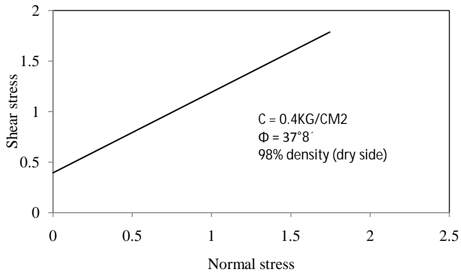
Figure 4.96 Shear stress vs normal stress for test -2, type- 1 soil
