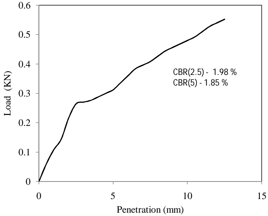
Figure 4.10 Load vs penetration graph for test -2, type -1 soil for soaked (day-1) condition
