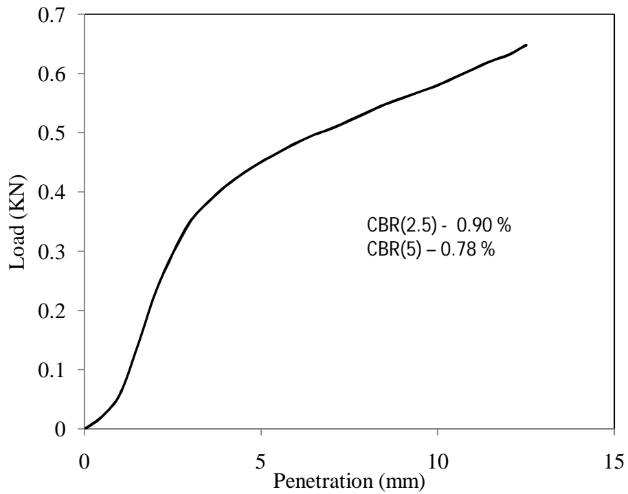
Figure 4.45 Load vs penetration graph for test -2, type -2 soil for soaked (day-5) condition
