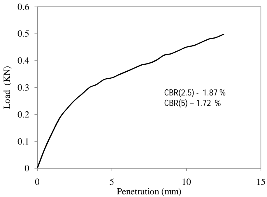
Figure 4.43 Load vs penetration graph for test -2, type -2 soil for soaked (day-3) condition
