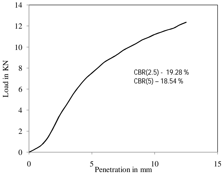
Figure 4.80 Load vs penetration graph for test -3, type - 3 soil for soaked (day - 3) condition
