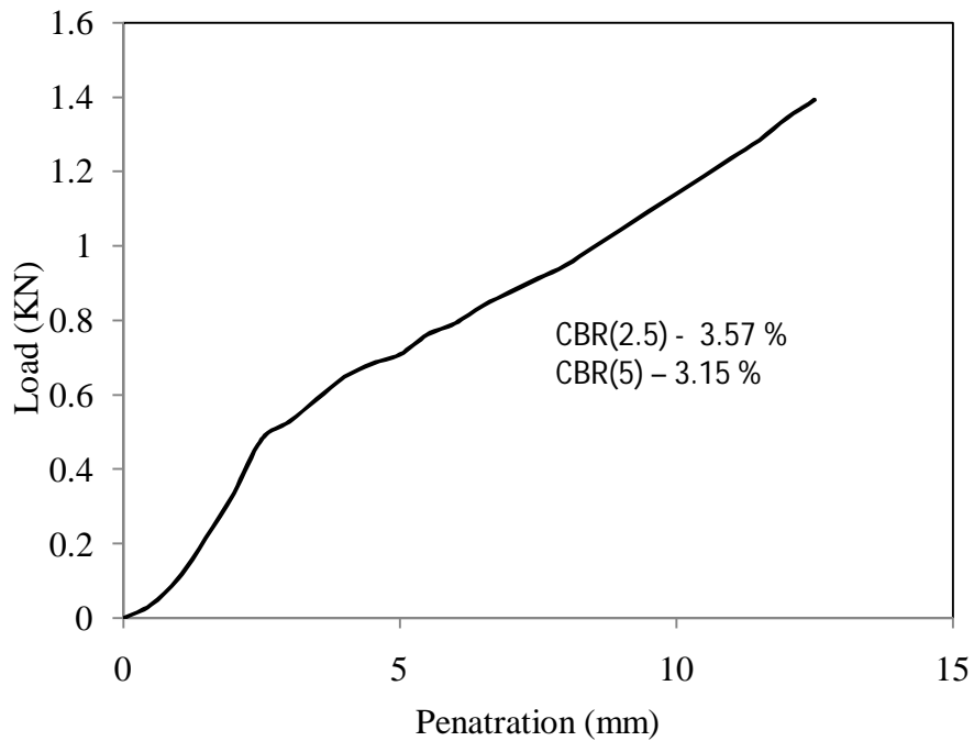
Figure 4.35 Load vs penetration graph for test -1, type - 2 soil for soaked (day-1) condition
