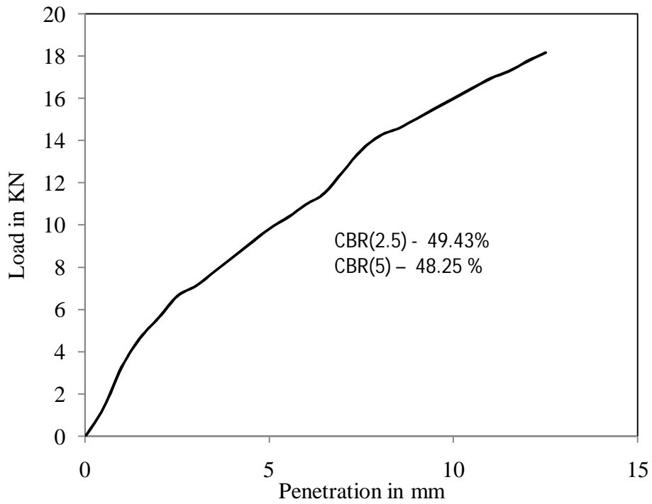
Figure 4.77 Load vs penetration graph for test -3, type - 3 soil for unsoaked condition
