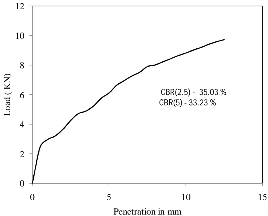
Figure 4.9 Load vs penetration graph for test –2, type – 1 soil for unsoaked condition
