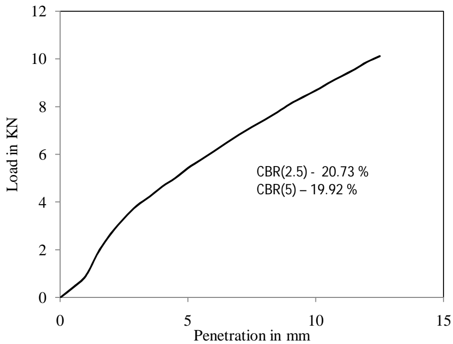
Figure 4.73 Load vs penetration graph for test -1, type - 3 soil for soaked (day-2) condition
