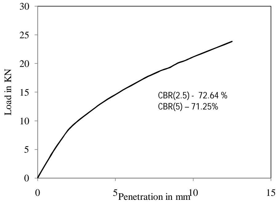
Figure 4.65 Load vs penetration graph for test -1, type -3 soil for unsoaked condition
