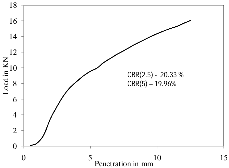
Figure 4.90 Load vs penetration graph for test -5, type -3 soil for soaked (day-1) condition
