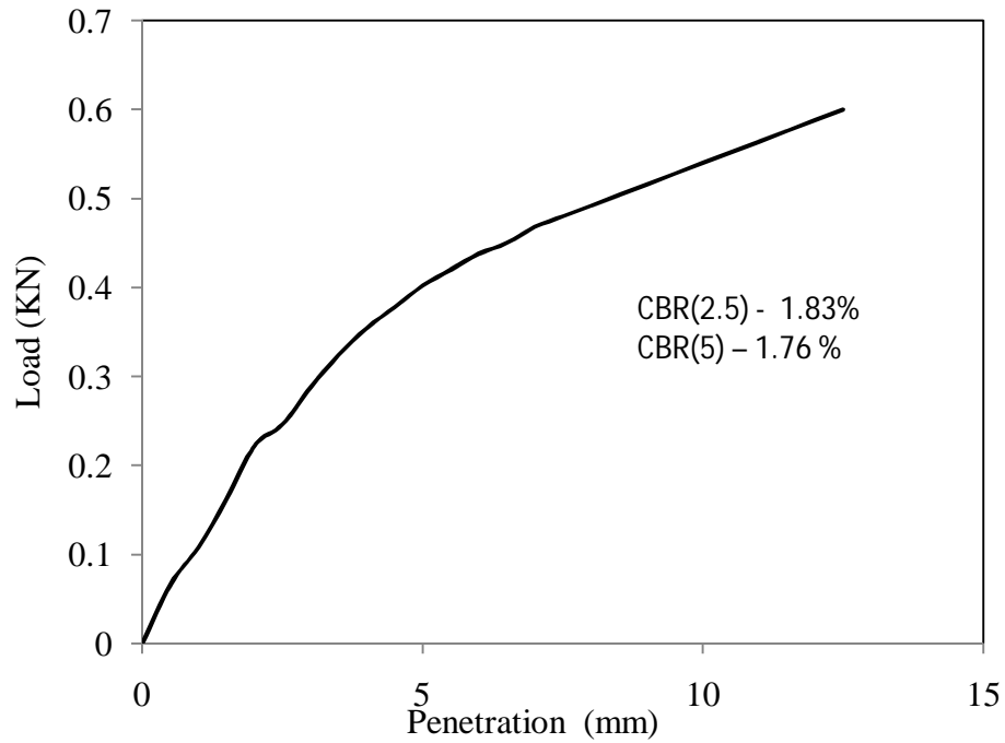
Figure 4.54 Load vs penetration graph for test -4, type -2 soil for soaked (day-2) condition
