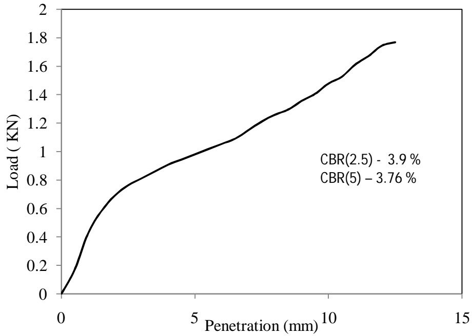
Figure 4.28 Load vs penetration graph for test -5, type -1 soil for soaked (day-1) condition
