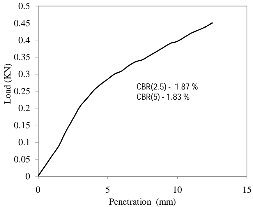
Figure 4.11 Load vs penetration graph for test -2, type -1 soil for soaked (day-2) condition
