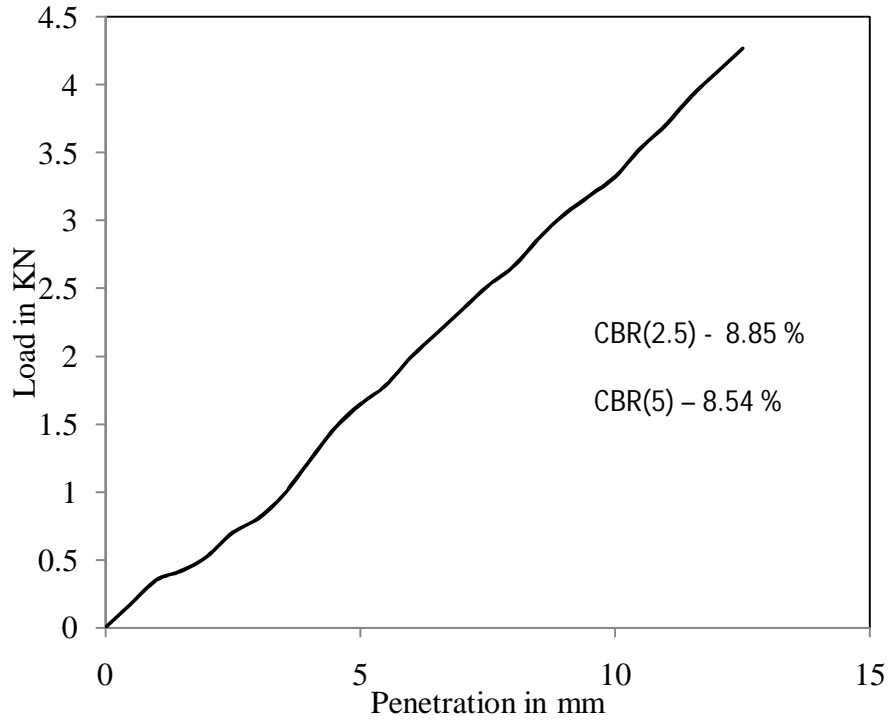
Figure 4.93 Load vs penetration graph for test -5, type -3 soil for soaked (day-4) condition
