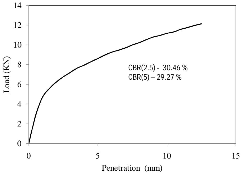
Figure 4.21 Load vs penetration graph for test -4, type -1 soil for unsoaked condition
