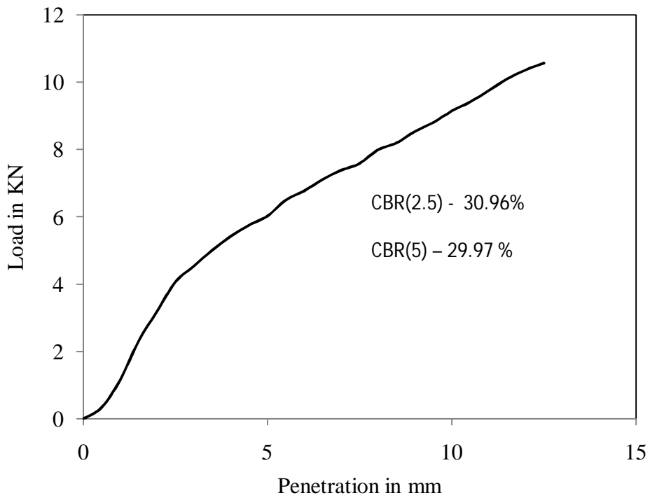
Figure 4.72 Load vs penetration graph for test -1, type -3 soil for soaked (day-1) condition
