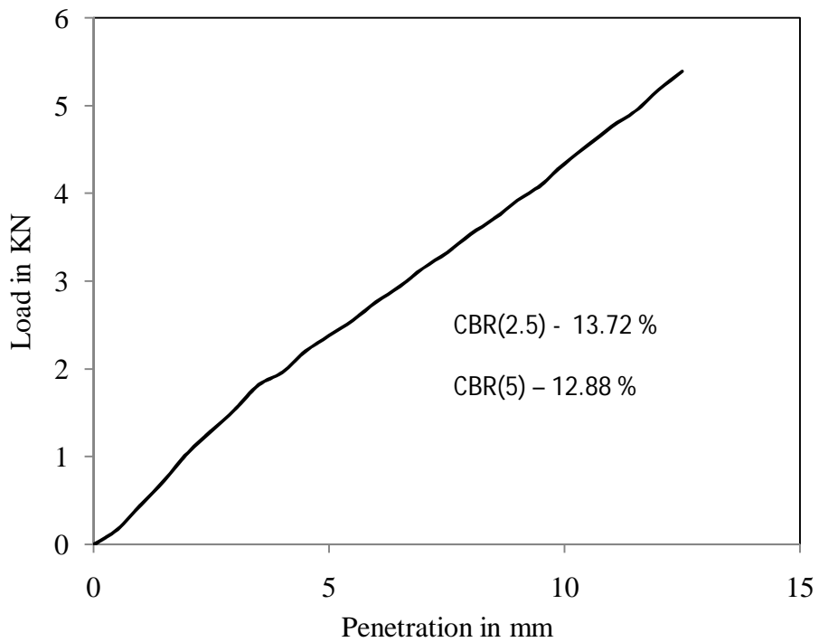
Figure 4.92 Load vs penetration graph for test -5, type -3 soil for soaked (day-3) condition
