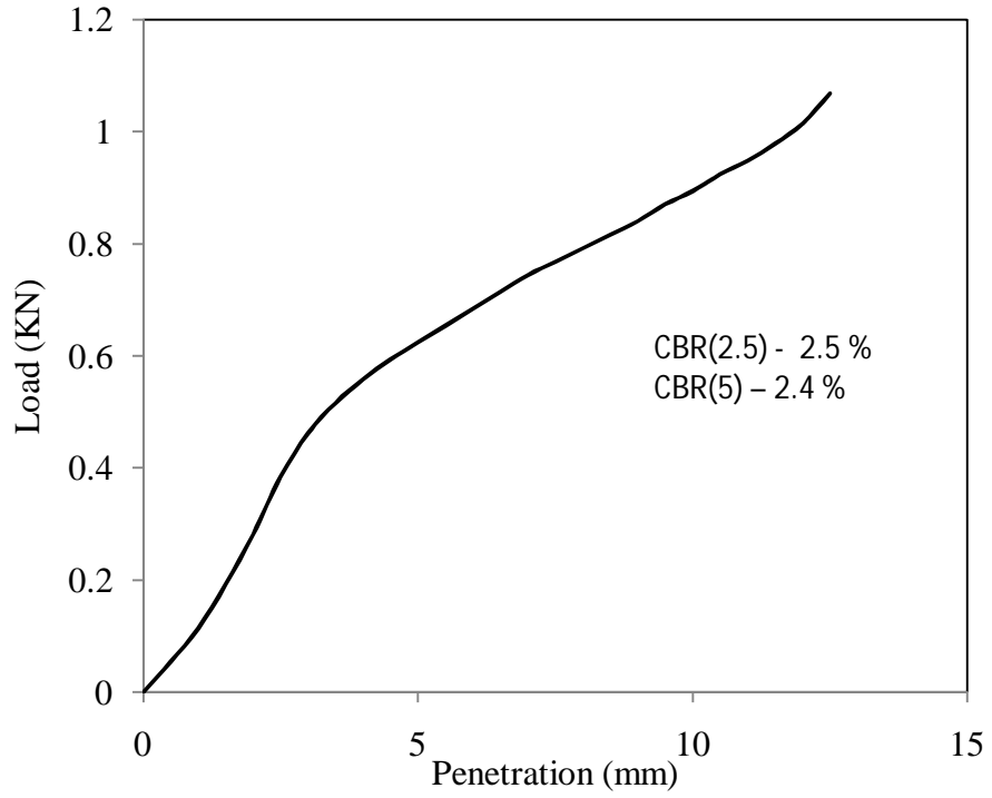
Figure 4.38 Load vs penetration graph for test -1, type -2 soil for soaked (day-4) condition
