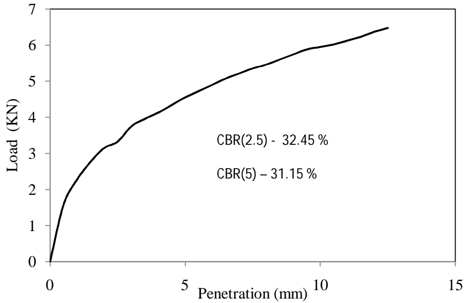
Figure 4.52 Load vs penetration graph for test -4, type -2 soil for unsoaked condition
