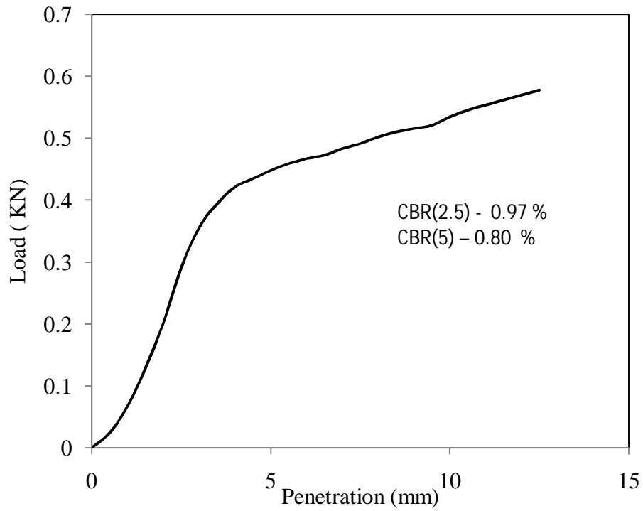
Figure 4.32 Load vs penetration graph for test -5, type -1 soil for soaked (day-5) condition
