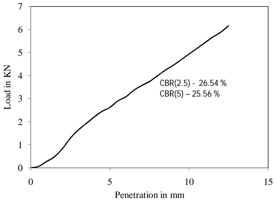
Figure 4.84 Load vs penetration graph for test -4, type -3 soil for soaked (day -1) condition
