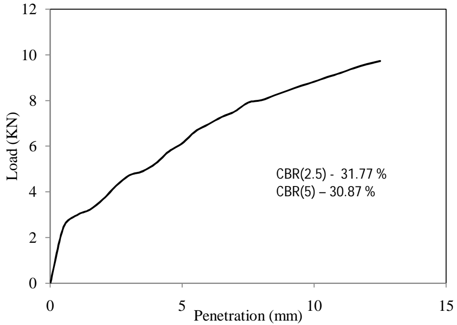
Figure 4.40 Load vs penetration graph for test -2, type - 2 soil for un soaked condition
