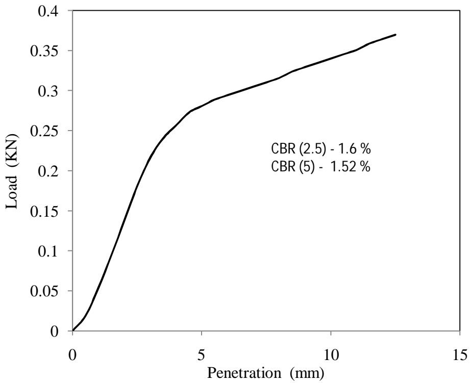
Figure 4.6 Load vs penetration graph for test -1, type - 1 soil for soaked (day - 4) condition
