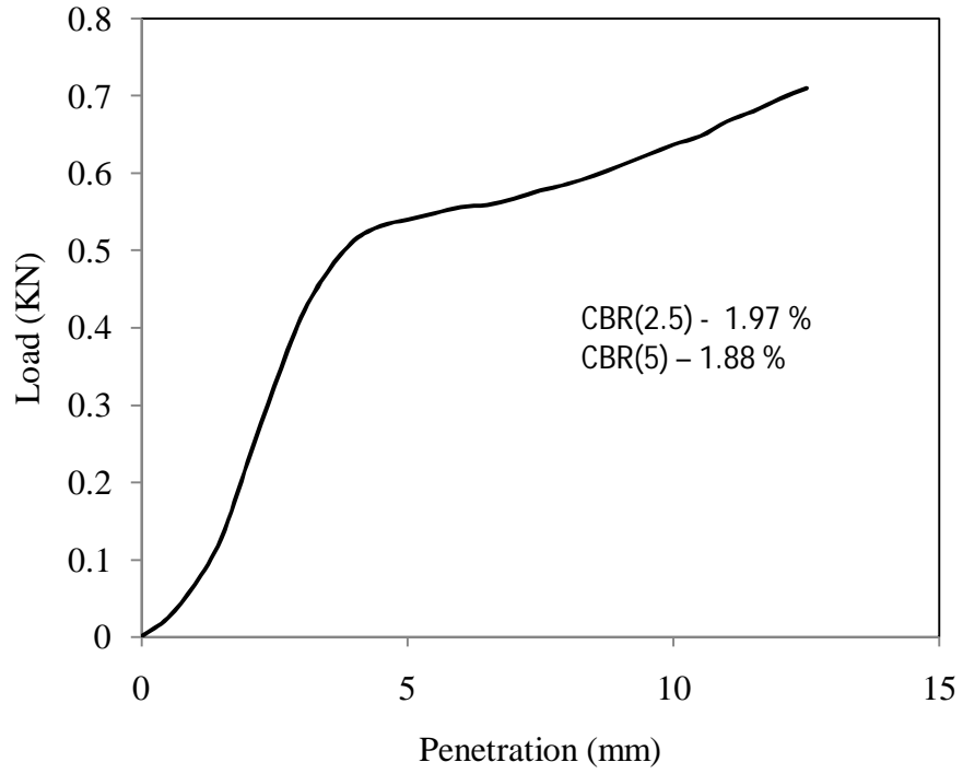
Figure 4.17 Load vs penetration graph for test -3, type -1 soil for soaked (day-2) condition
