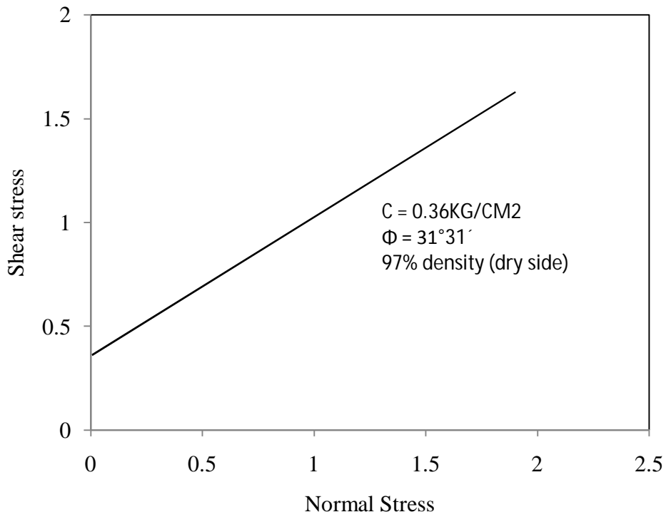
Figure 4.98 Shear stress vs normal stress for test -4, type- 1 soil
