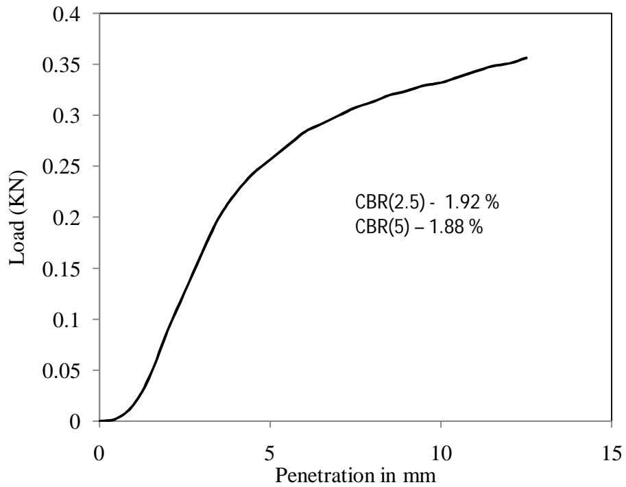
Figure 4.26 Load vs penetration graph for test -4, type -1 soil for soaked (day-5) condition
