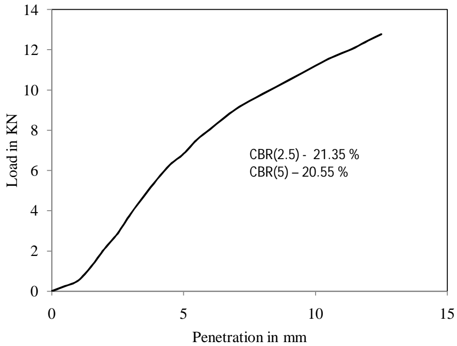
Figure 4.68 Load vs penetration graph for test -1, type - 3 soil for soaked (day-3) condition
