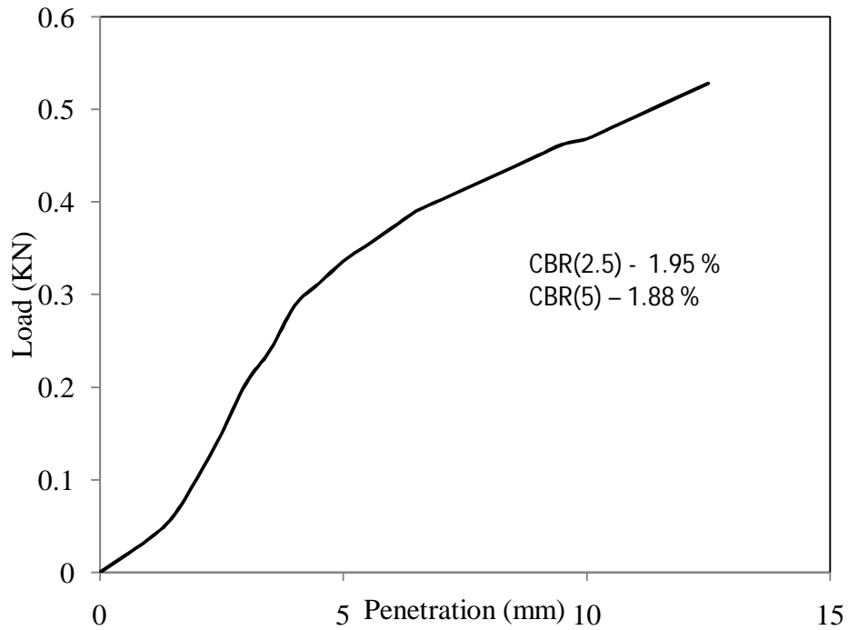
Figure 4.48 Load vs penetration graph for test -3, type - 2 soil for soaked (day-2) condition
