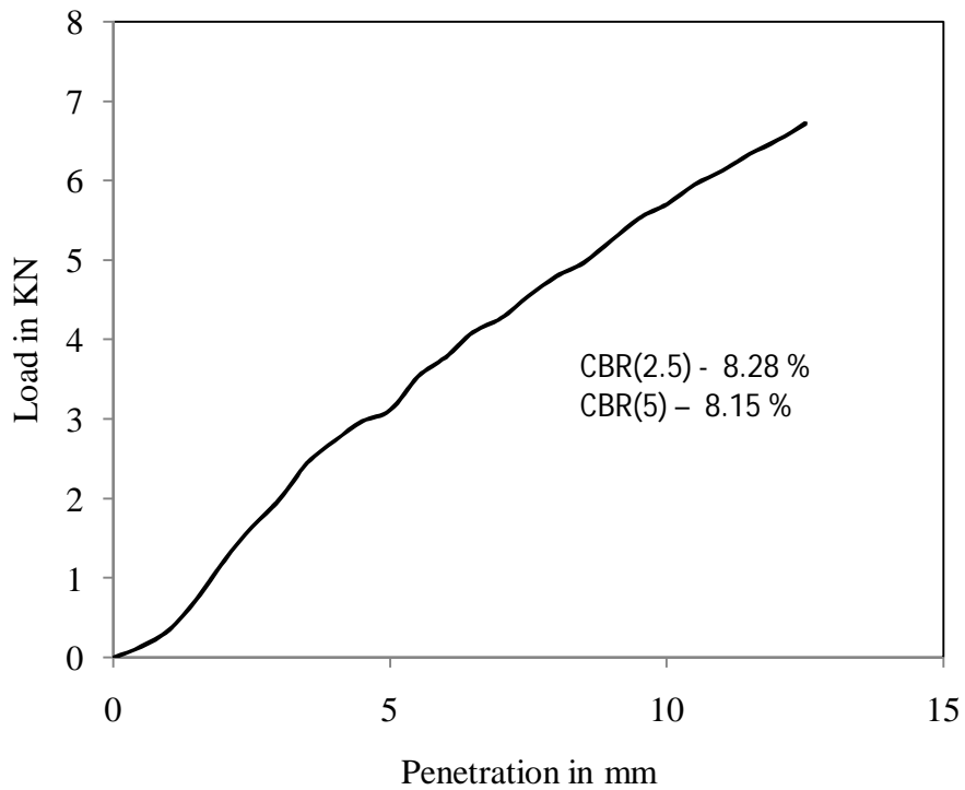
Figure 4.94 Load vs penetration graph for test -5, type -3 soil for soaked (day-5) condition
