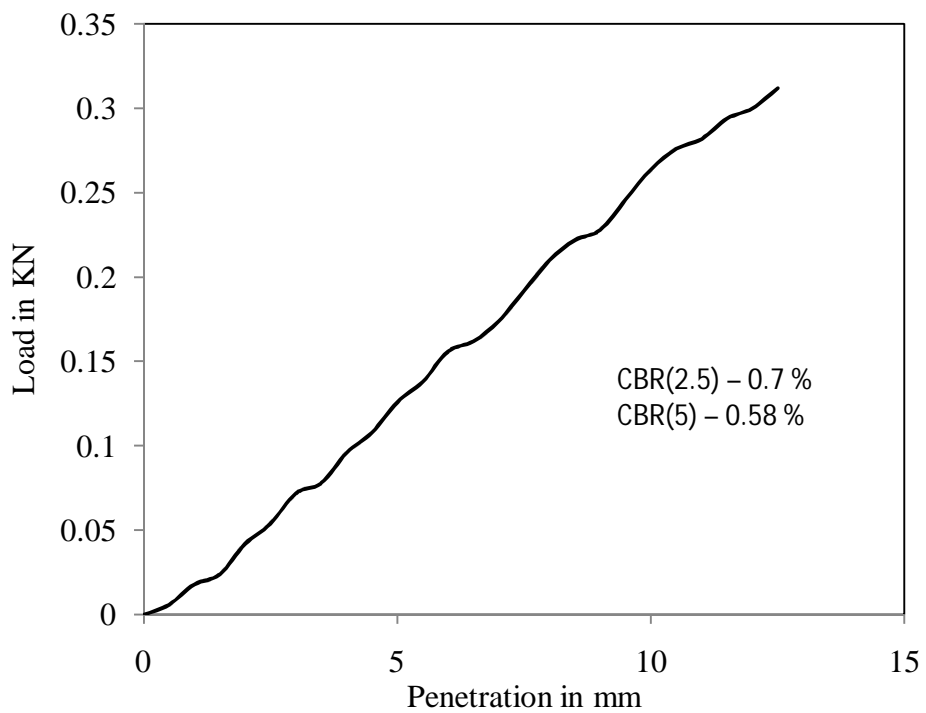
Figure 4.57 Load vs penetration graph for test -4, type -2 soil for soaked (day-5) condition
