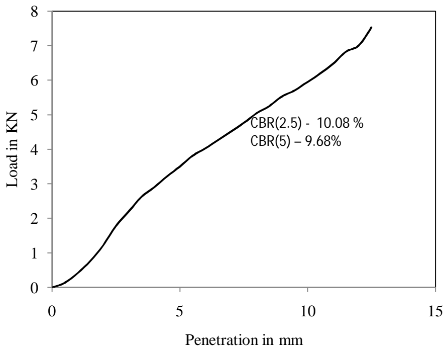
Figure 4.88 Load vs penetration graph for test -4, type - 3 soil for soaked (day-5) condition
