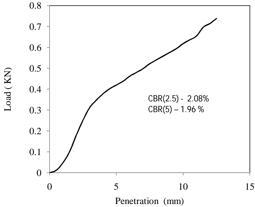
Figure 4.48 Load vs penetration graph for test -3, type - 2 soil for soaked (day-2) condition
