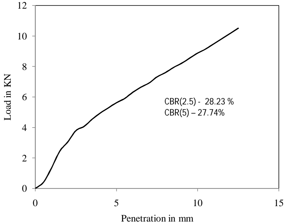
Figure 4.79 Load vs penetration graph for test -3, type - 3 soil for soaked (day - 2) condition
