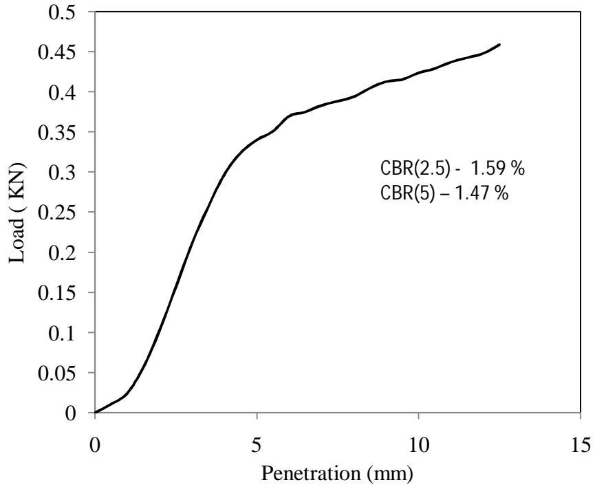
Figure 4.19 Load vs penetration graph for test -3, type -1 soil for soaked (day-4) condition
