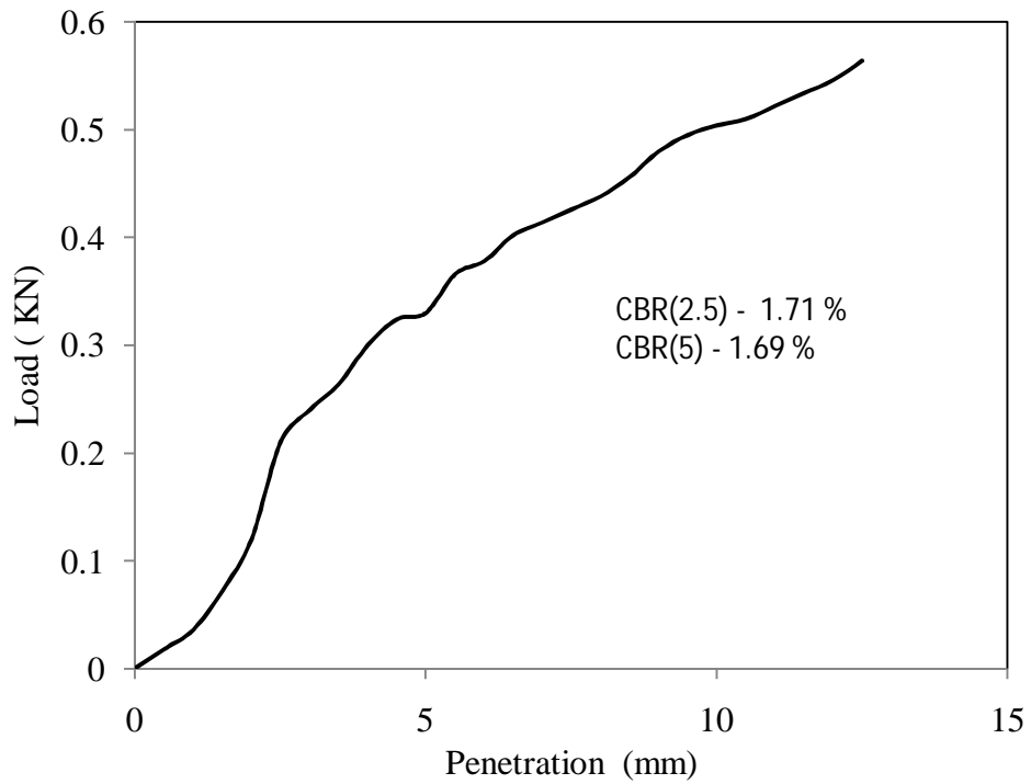
Figure 4.13 Load vs penetration graph for test -2, type -1 soil for soaked (day-4) condition
