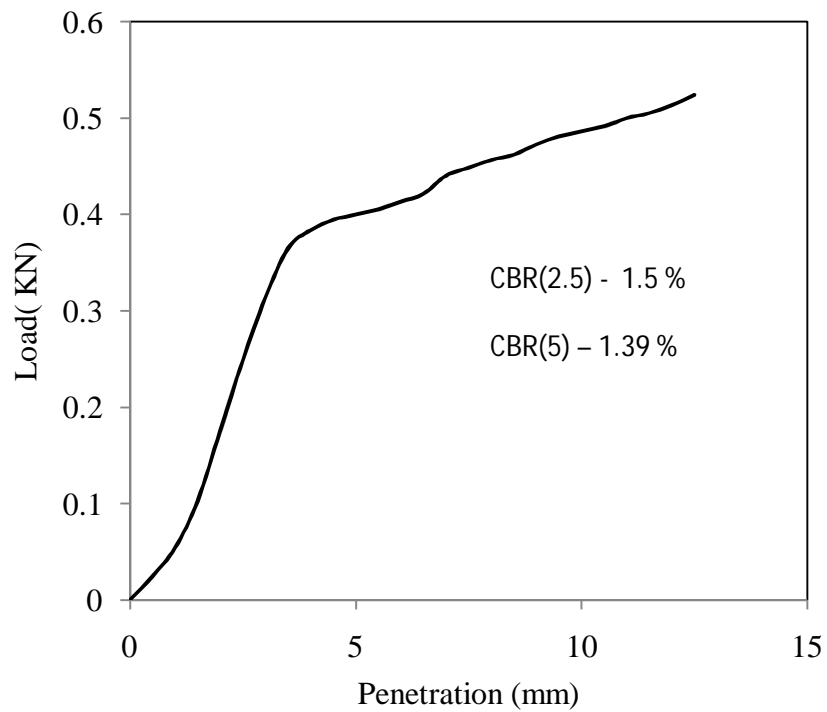
Figure 4.30 Load vs penetration graph for test -5, type -1 soil for soaked (day-3) condition
