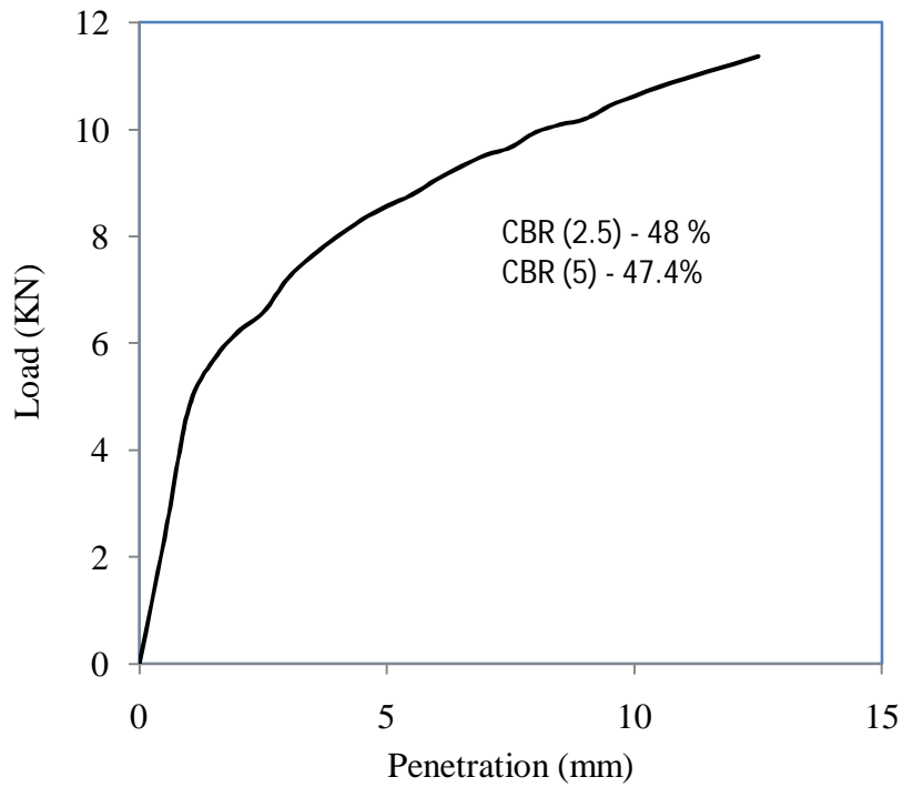
Figure 4.2 Load vs penetration graph for test – 1, type – 1 soil for unsoaked condition
