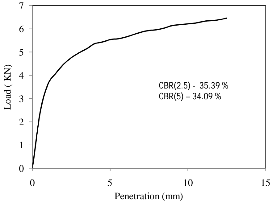
Figure 4.34 Load vs penetration graph for test -1, type - 2 soil for unsoaked condition
