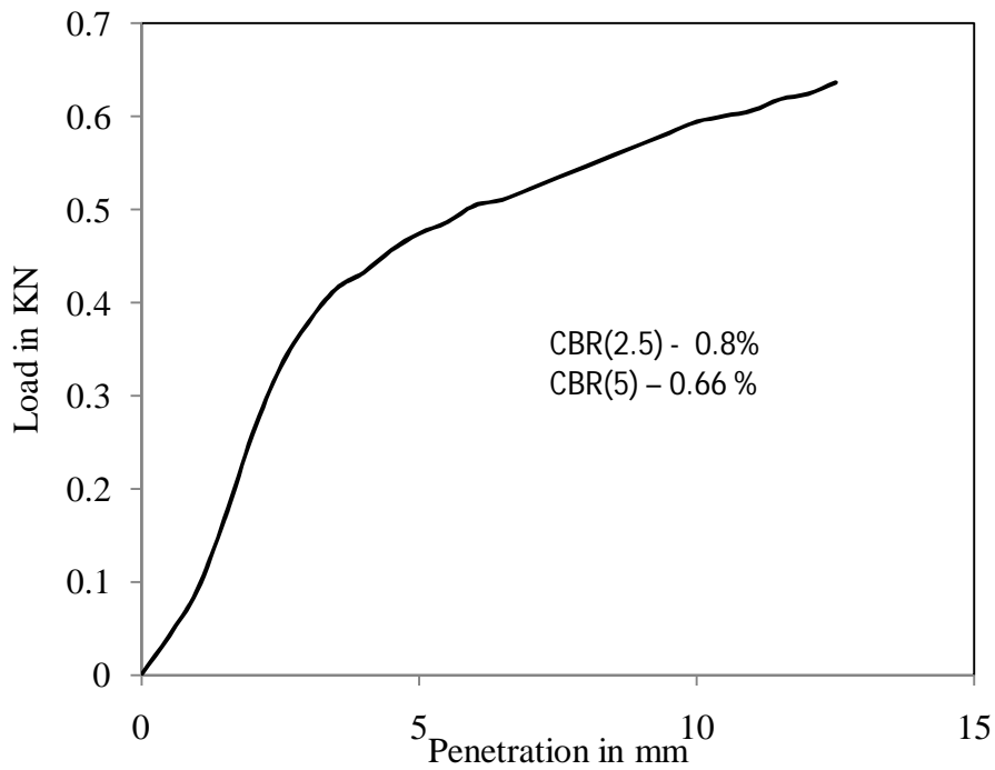
Figure 4.63 Load vs penetration graph for test -5, type - 2 soil for soaked (day-5) condition
