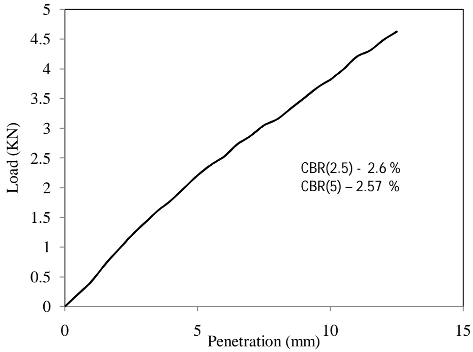
Figure 4.42 Load vs penetration graph for test -2, type -2 soil for soaked (day-2) condition
