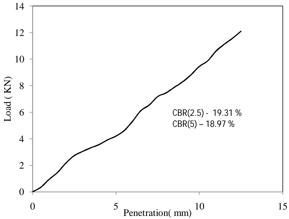
Figure 4.70 Load vs penetration graph for test -1, type - 3 soil for soaked (day-5) condition
