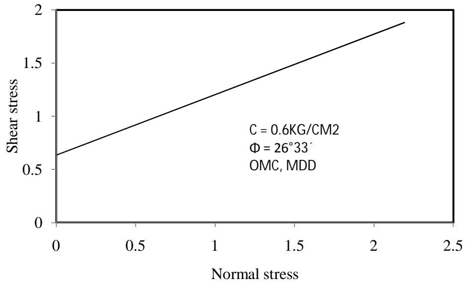
Figure 4.95 Shear stress vs normal stress for test -1, type- 1 soil
