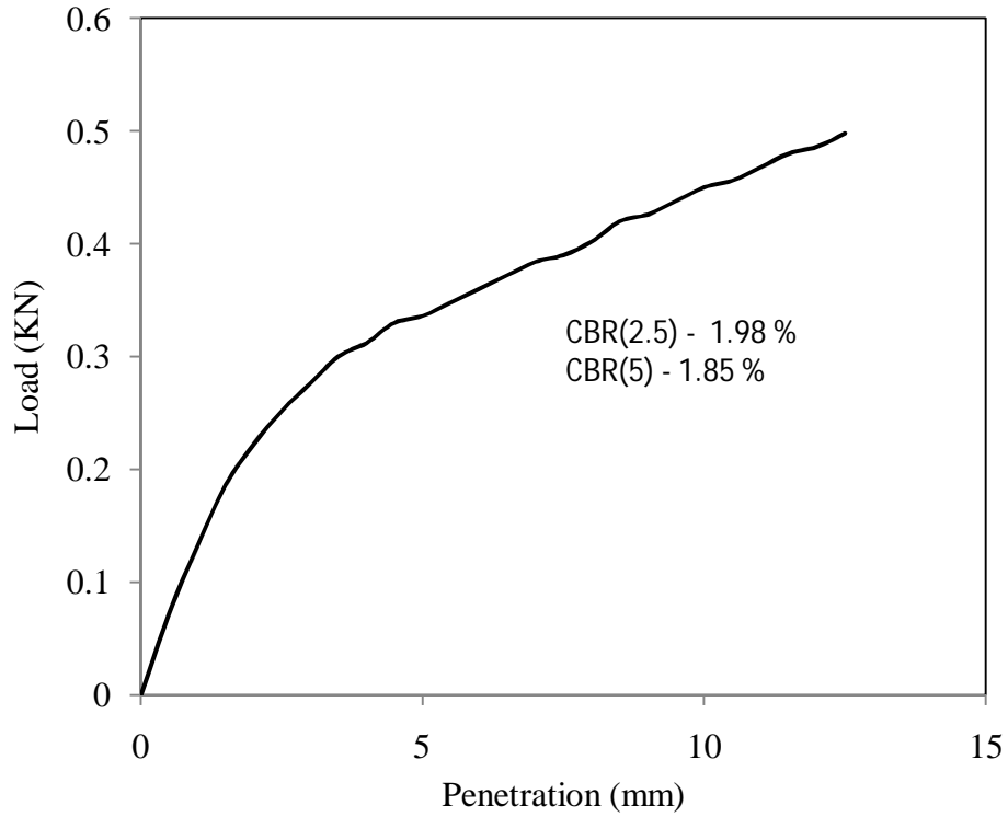
Figure 4.12 Load vs penetration graph for test -2, type -1 soil for soaked (day-3) condition
