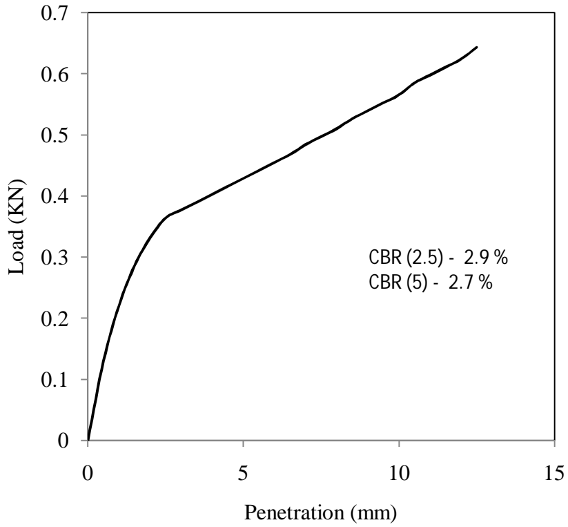
Figure 4.3 Load vs penetration graph for test -1, type - 1soil for soaked (day - 1) condition
