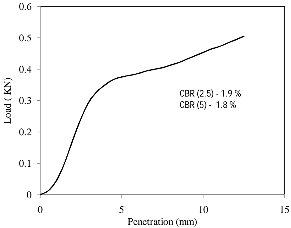
Figure 4.5 Load vs penetration graph for test -1, type - 1 soil for soaked (day - 3) condition
