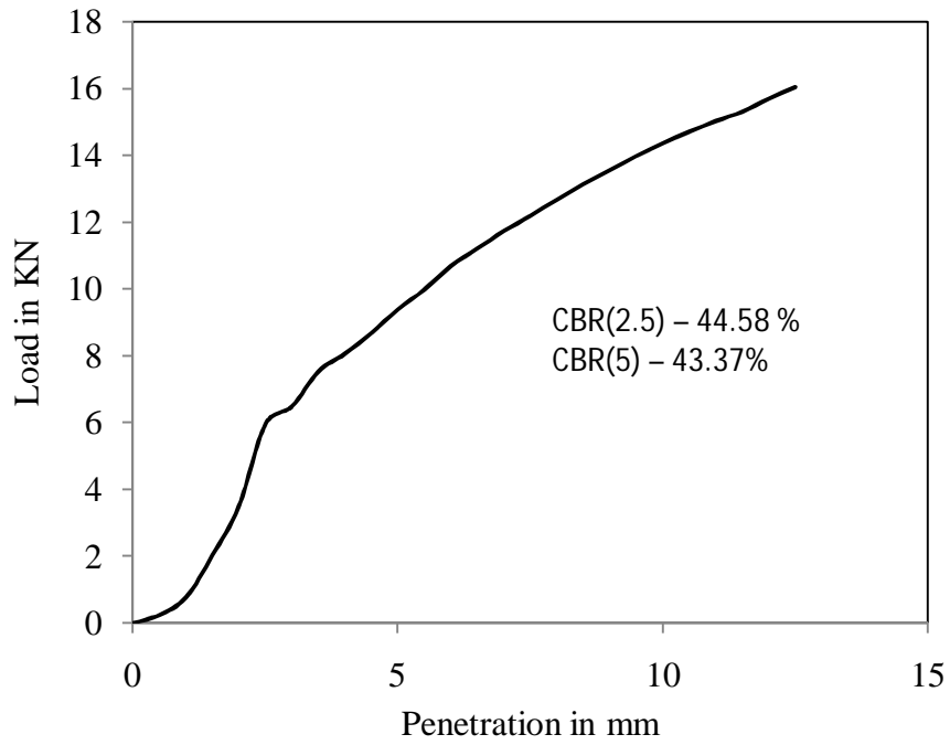
Figure 4.71 Load vs penetration graph for test -1, type -3 soil for unsoaked condition
