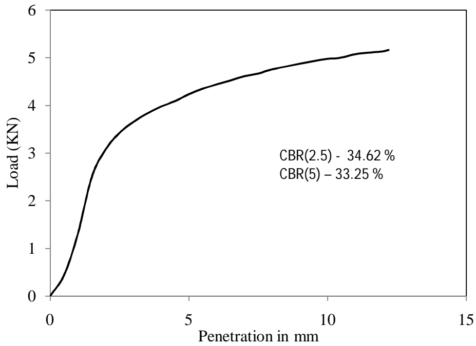
Figure 4.27 Load vs penetration graph for test -5, type -1 soil for unsoaked condition
