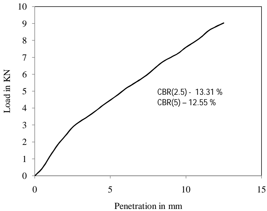
Figure 4.82 Load vs penetration graph for test -3, type - 3 soil for soaked (day - 5) condition
