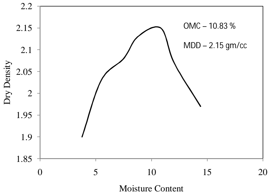
Figure 4.64 Modified proctor compaction test for type – 3 soil
