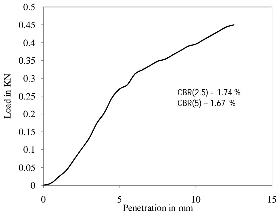
Figure 4.55 Load vs penetration graph for test -4, type -2 soil for soaked (day-3) condition
