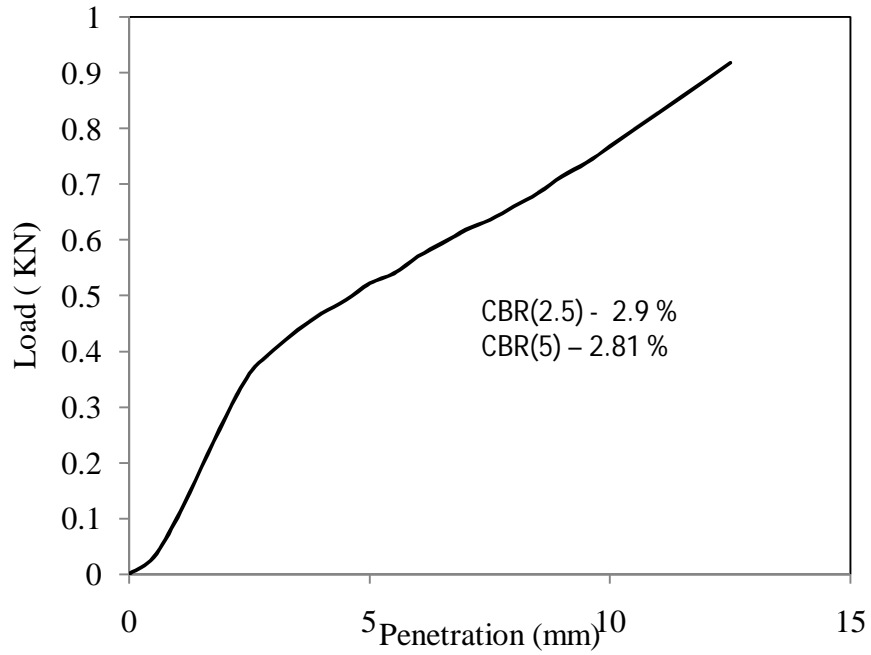
Figure 4.36 Load vs penetration graph for test -1, type -2 soil for soaked (day-2) condition
