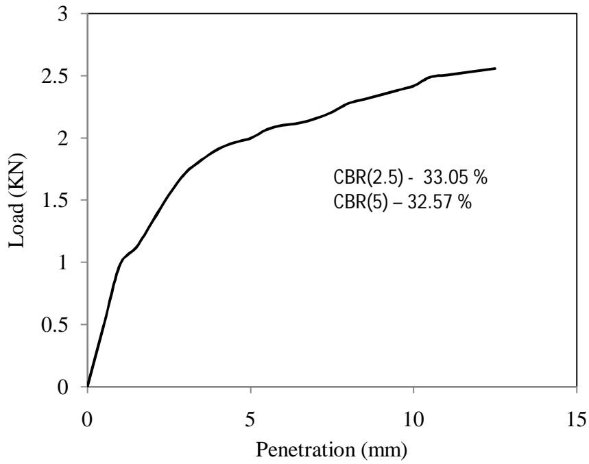
Figure 4.46 Load vs penetration graph for test -3, type -2 soil for unsoaked condition
