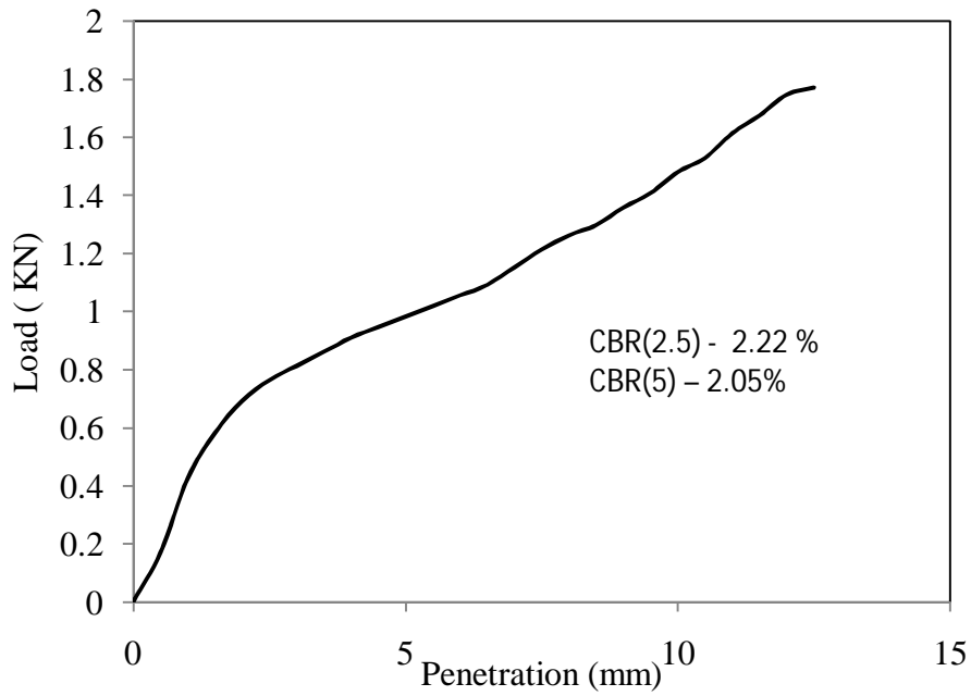
Figure 4.16 Load vs penetration graph for test -3, type -1 soil for soaked (day-1) condition
