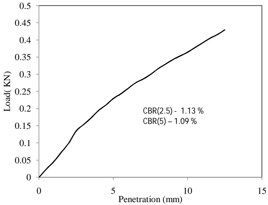
Figure 4.39 Load vs penetration graph for test -1, type -2 soil for soaked (day-5) condition
