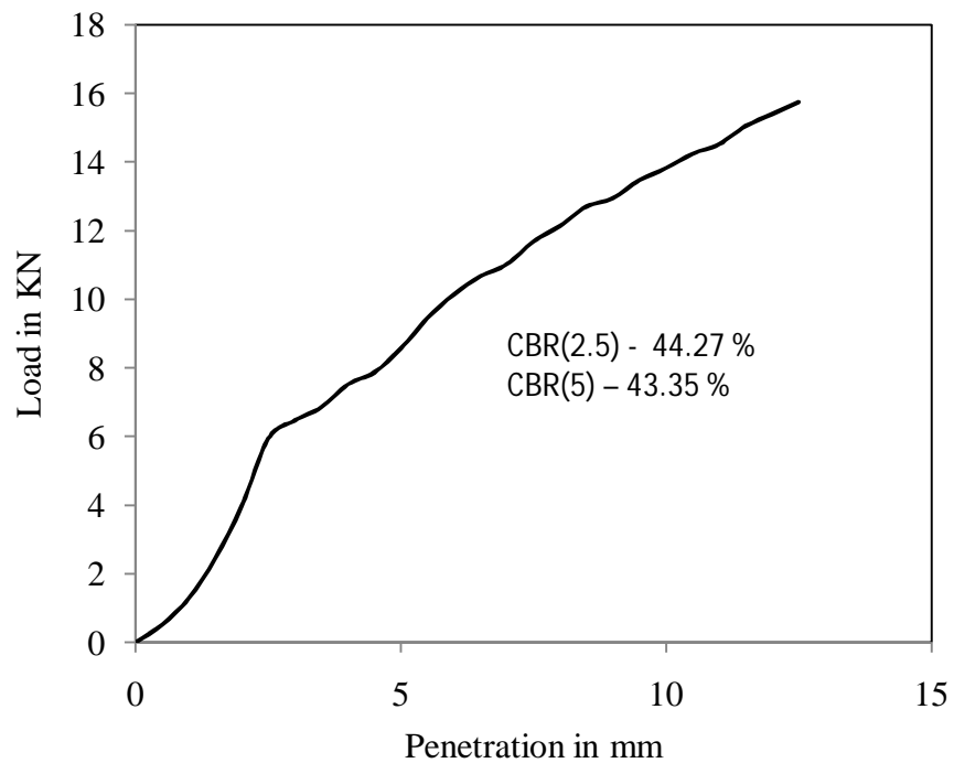
Figure 4.66 Load vs penetration graph for test -1, type -3 soil for soaked (day-1) condition
