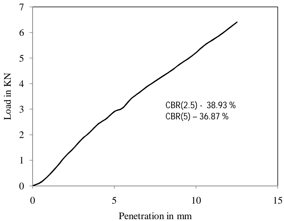
Figure 4.78 Load vs penetration graph for test -3, type - 3 soil for soaked (day - 1) condition
