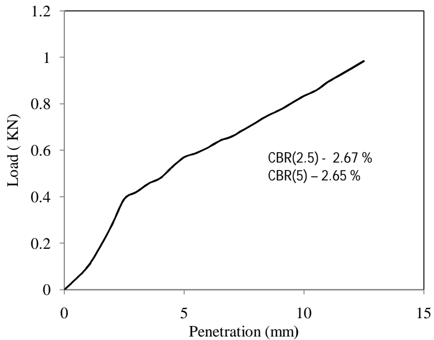
Figure 4.37 Load vs penetration graph for test -1, type -2 soil for soaked (day-3) condition
