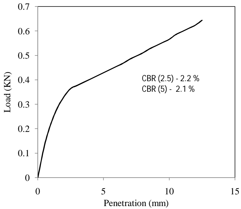
Figure 4.4 Load vs penetration graph for test -1, type - 1soil for soaked (day - 2) condition
