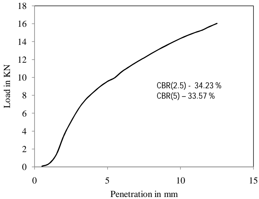
Figure 4.89 Load vs penetration graph for test -5, type -3 soil for unsoaked condition
