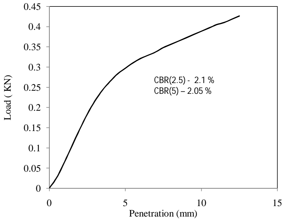
Figure 4.24 Load vs penetration graph for test -4, type -1 soil for soaked (day-3) condition
