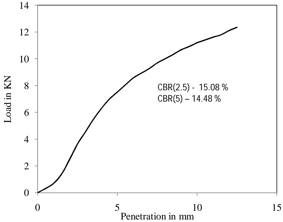
Figure 4.75 Load vs penetration graph for test -1, type - 3 soil for soaked (day-4) condition
