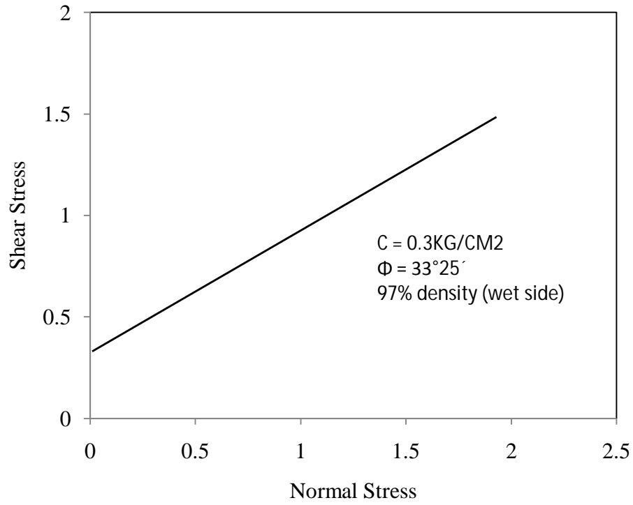
Figure 4.99 Shear stress vs normal stress for test -5, type- 1 soil
