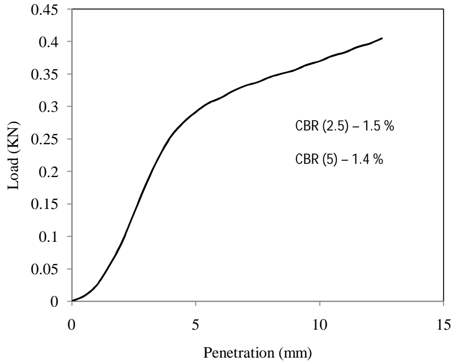
Figure 4.7 Load vs penetration graph for test -1, type - 1 soil for soaked (day - 5) condition
