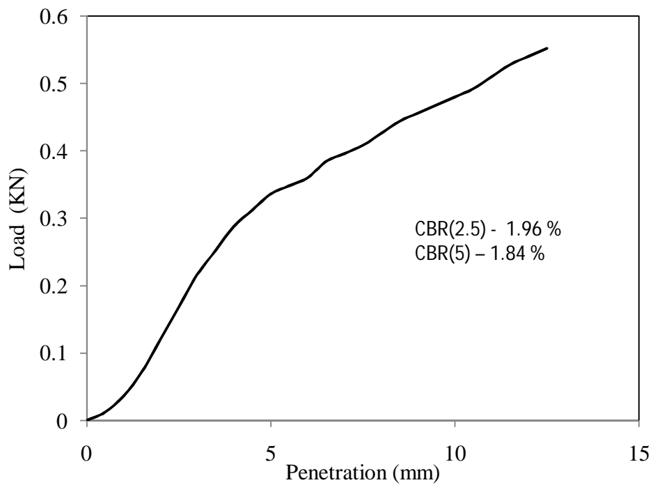
Figure 4.41 Load vs penetration graph for test -2, type - 2 soil for soaked (day-1) condition
