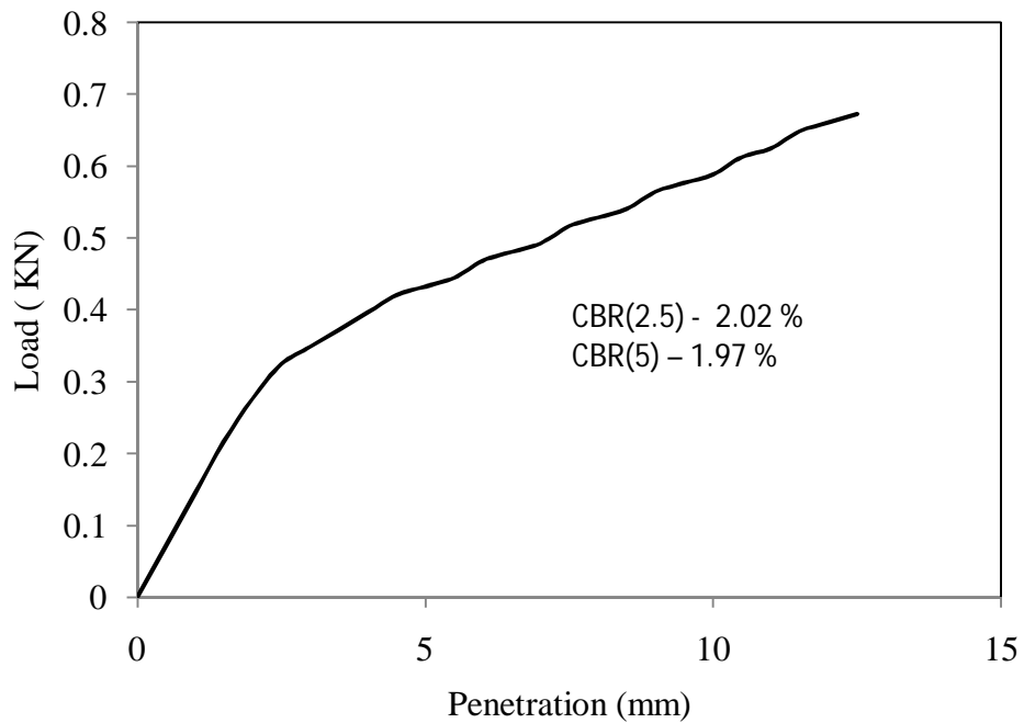
Figure 4.53 Load vs penetration graph for test -4, type -2 soil for soaked (day-1) condition
