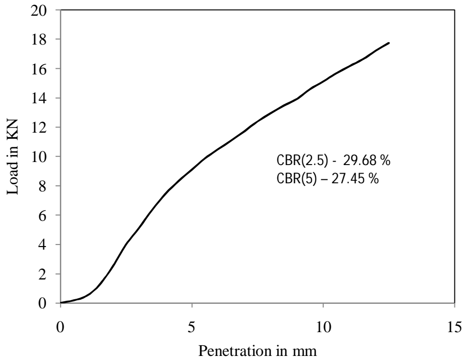
Figure 4.67 Load vs penetration graph for test -1, type - 3 soil for soaked (day-2) condition
