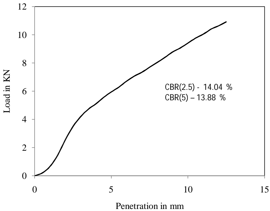
Figure 4.76 Load vs penetration graph for test -1, type - 3 soil for soaked (day-5) condition
