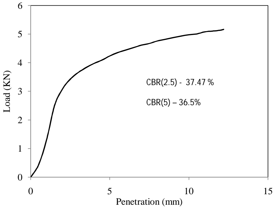
Figure 4.15 Load vs penetration graph for test -3, type -1 soil for unsoaked condition
