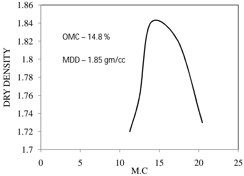
Figure 4.33: Modified proctor compaction test for type – 2 soil
