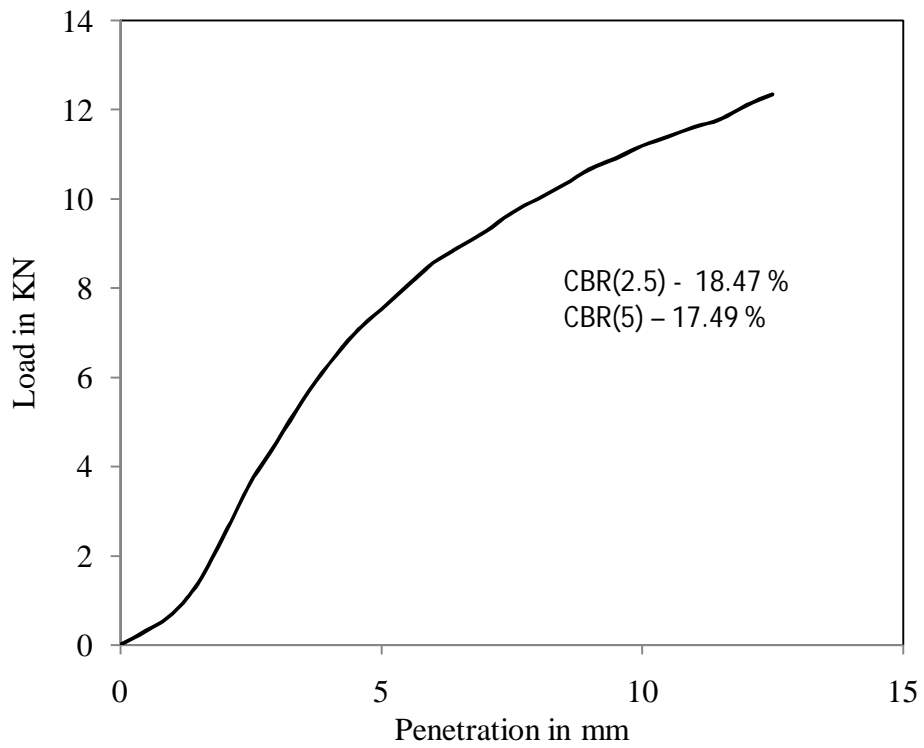
Figure 4.86 Load vs penetration graph for test -4, type - 3 soil for soaked (day-3) condition
