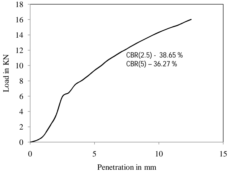
Figure 4.83 Load vs penetration graph for test -4, type -3 soil for unsoaked condition
