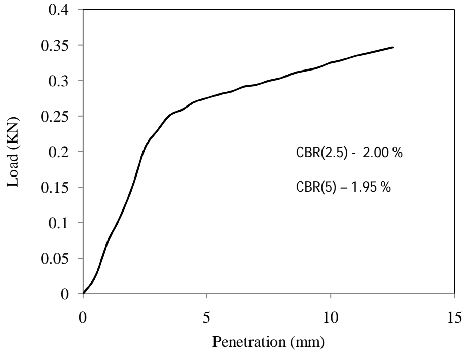
Figure 4.25 Load vs penetration graph for test -4, type -1 soil for soaked (day-4) condition
