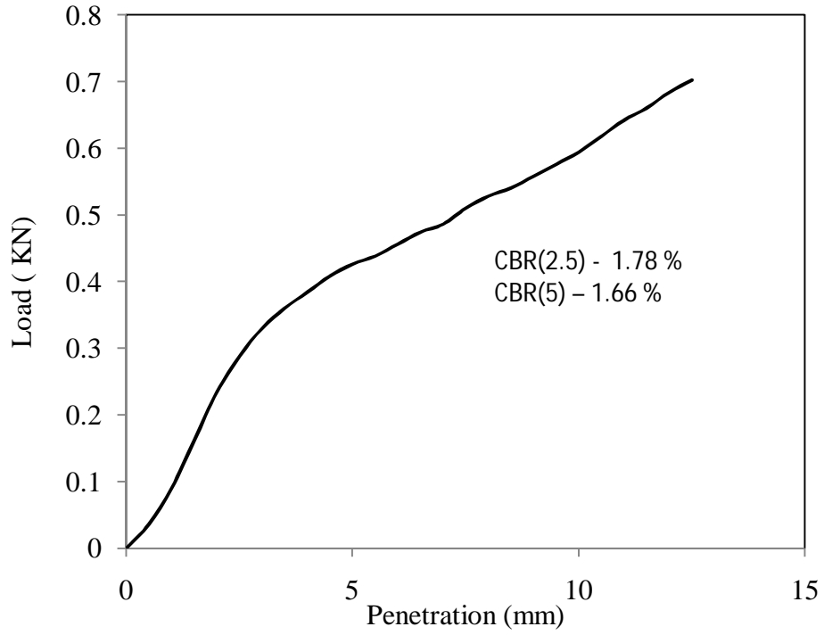
Figure 4.50 Load vs penetration graph for test -3, type -2 soil for soaked (day-4) condition
