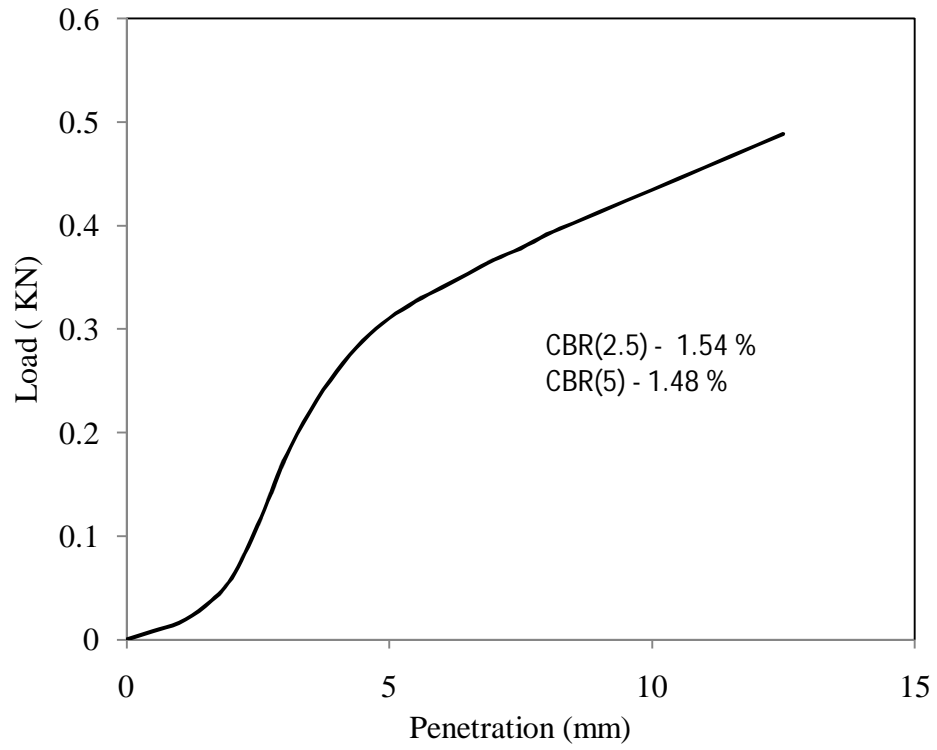
Figure 4.14 Load vs penetration graph for test -2, type - 1 soil for soaked (day-5) condition
