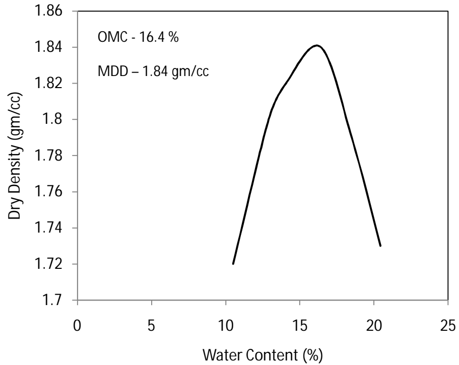
Figure 4.1: Modified proctor compaction test for type – 1 soil
