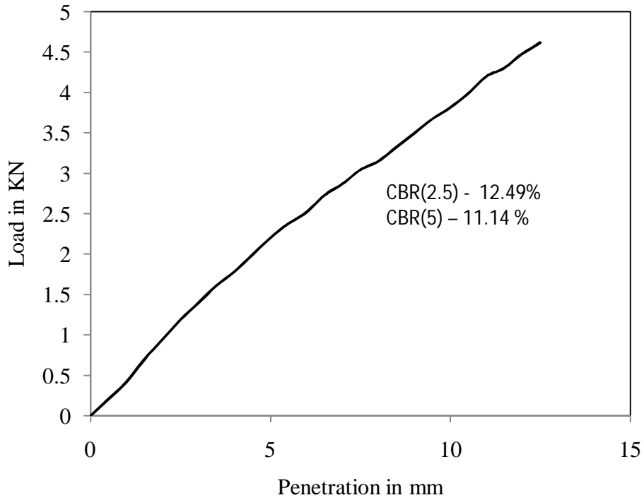
Figure 4.87 Load vs penetration graph for test -4, type - 3 soil for soaked (day-5) condition
