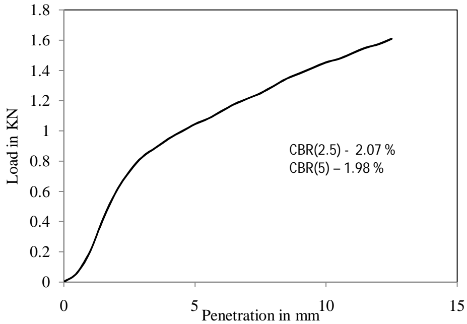
Figure 4.59 Load vs penetration graph for test -5, type -2 soil for soaked (day-1) condition
