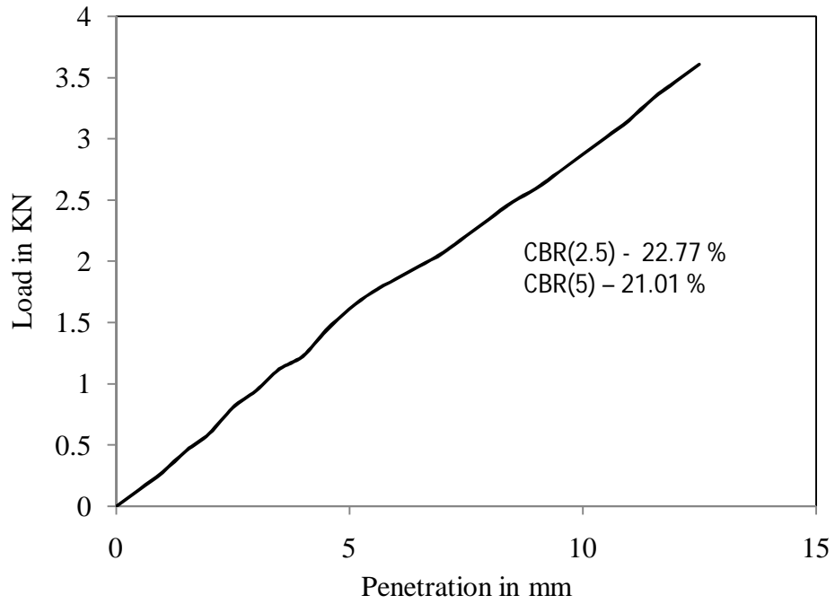
Figure 4.85 Load vs penetration graph for test -4, type - 3 soil for soaked (day-2) condition
