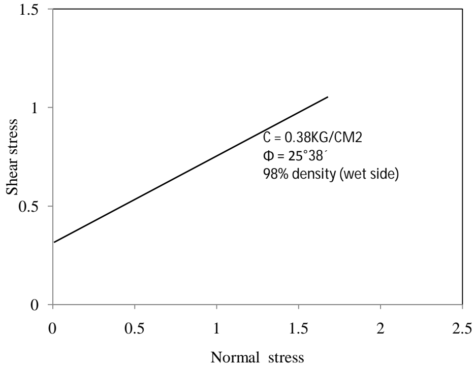
Figure 4.97 Shear stress vs normal stress for test -3, type- 1 soil
