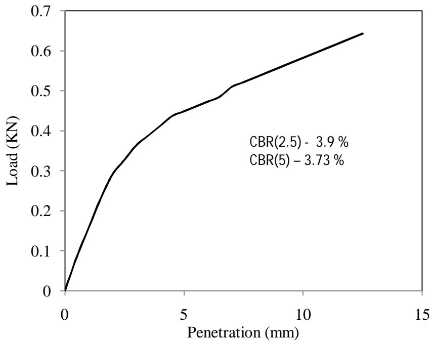
Figure 4.22 Load vs penetration graph for test -4, type -1 soil for soaked (day-1) condition
