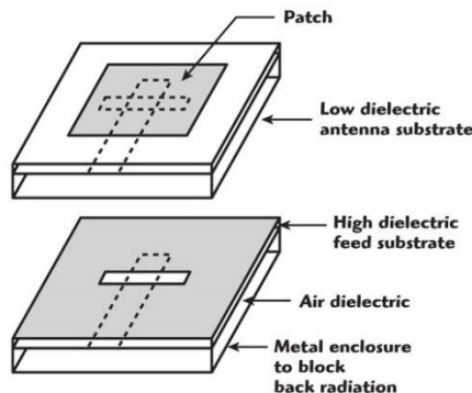
Figure 7 Dielectric Image Guide Coupling
