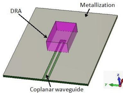
Figure 6 Coplanar Coupling
