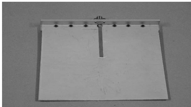
Figure 4 Aperture Coupling [3]
