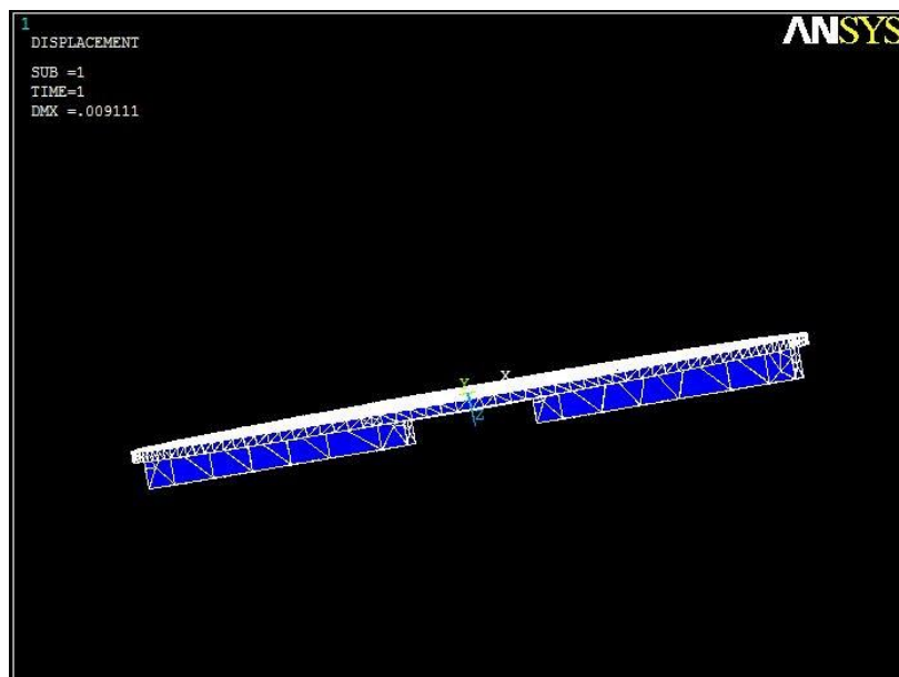
Figure 4.11 Deflection profile of plate with one stiffener
