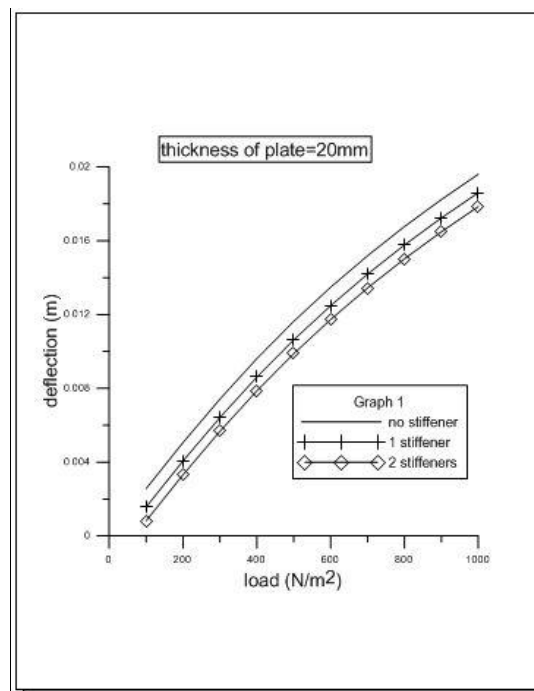
Figure 4.9 Load vs. deflection of annular plates of thickness 20mm with stiffeners
