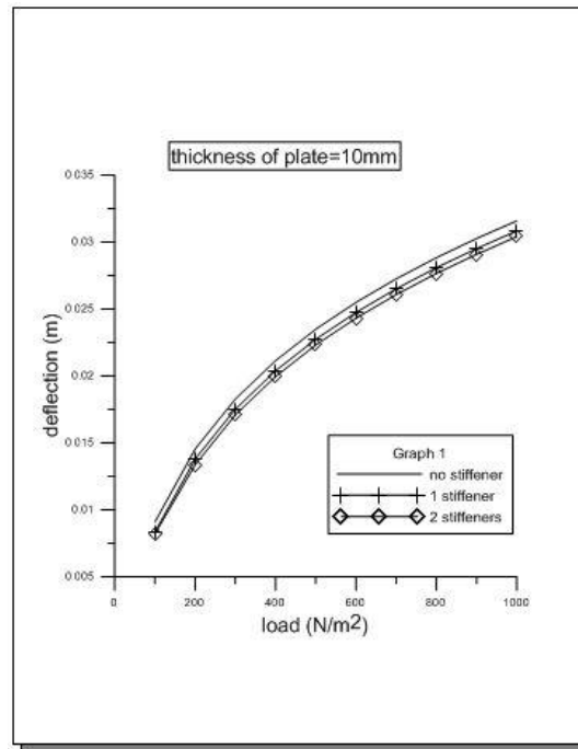
Figure 4.10 Load Vs. deflection of annular plates with thickness 10mm with stiffeners
