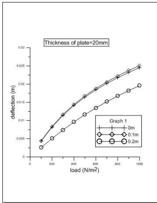
Figure 4.2 Load vs deflection for 20mm plate
