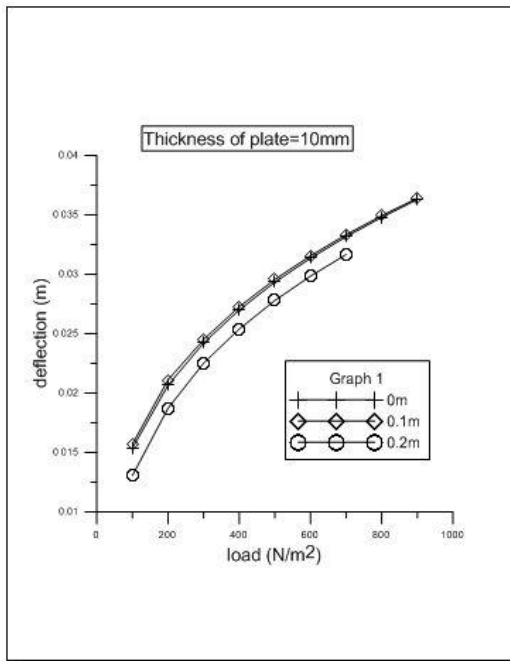
Figure 4.4 Load vs deflection for 10 mm plate
