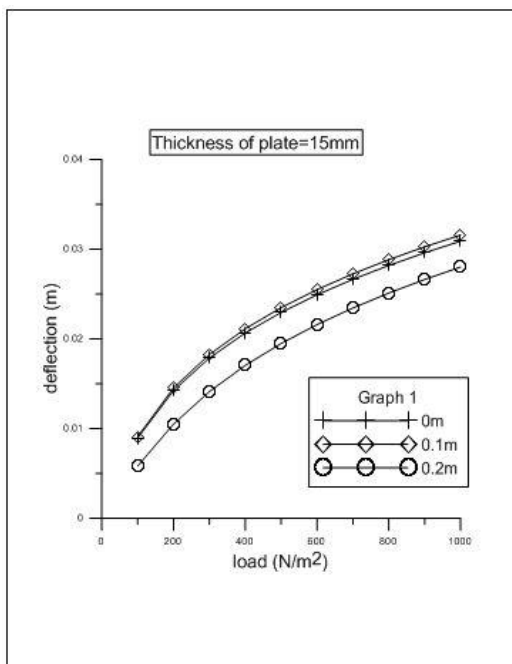
Figure 4.3 Load vs deflection for 15 mm plate
