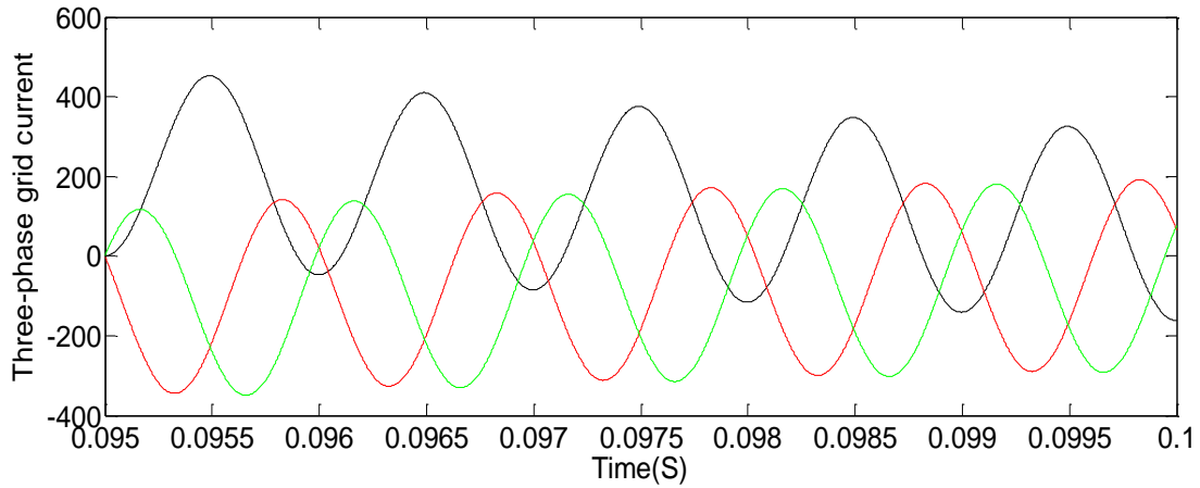
Fig 3.5 shows the relationship between 3-phase grids current
