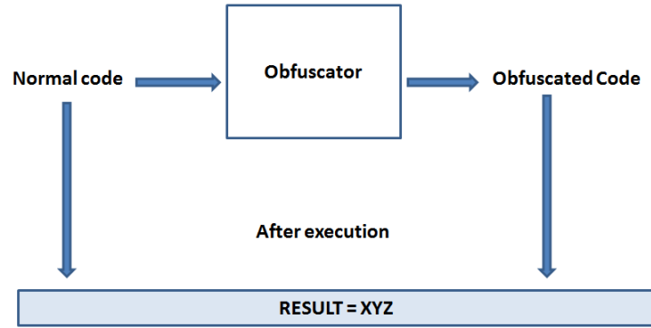
Figure 2.5: Code Obfuscation
