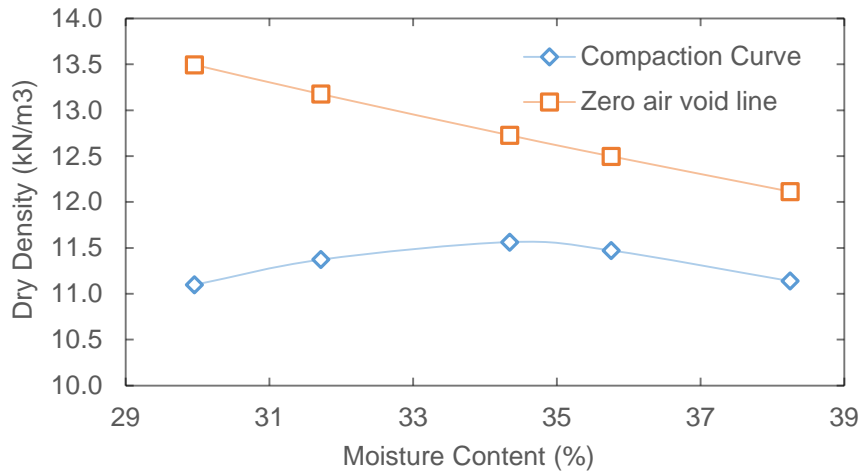
Figure 3.4. Light Compaction curve for Fly ash
