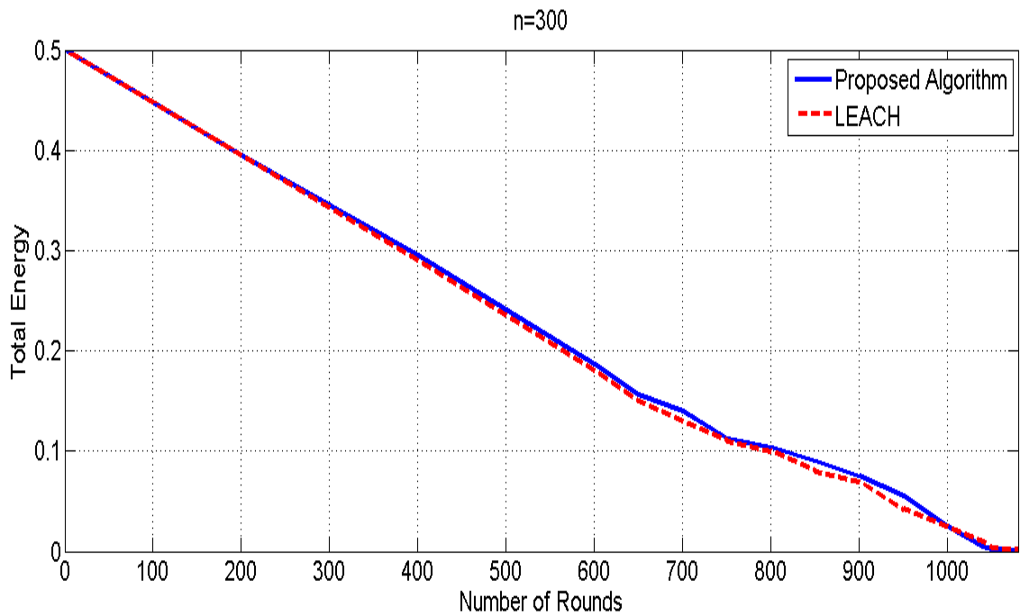
Figure 4.4: Energy dissipation for 300 nodes
