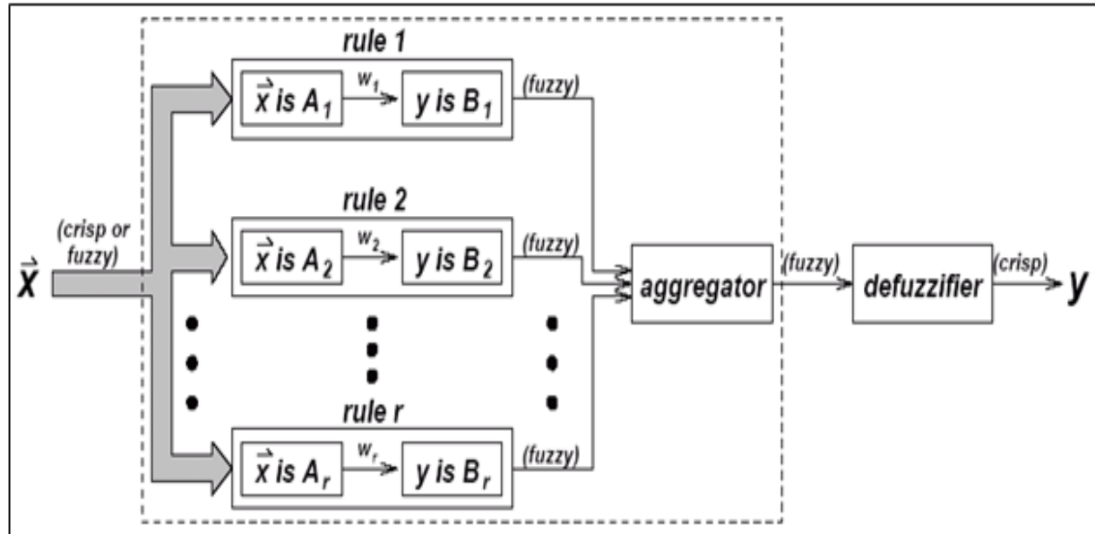
Fig.4.3: Inference Engine
